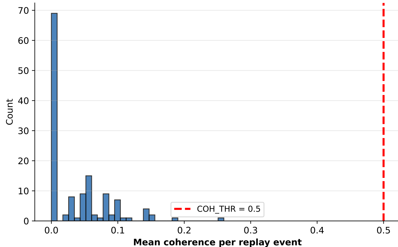
Replay Coherence Distribution (n=135 events) max=0.260, threshold=0.5
