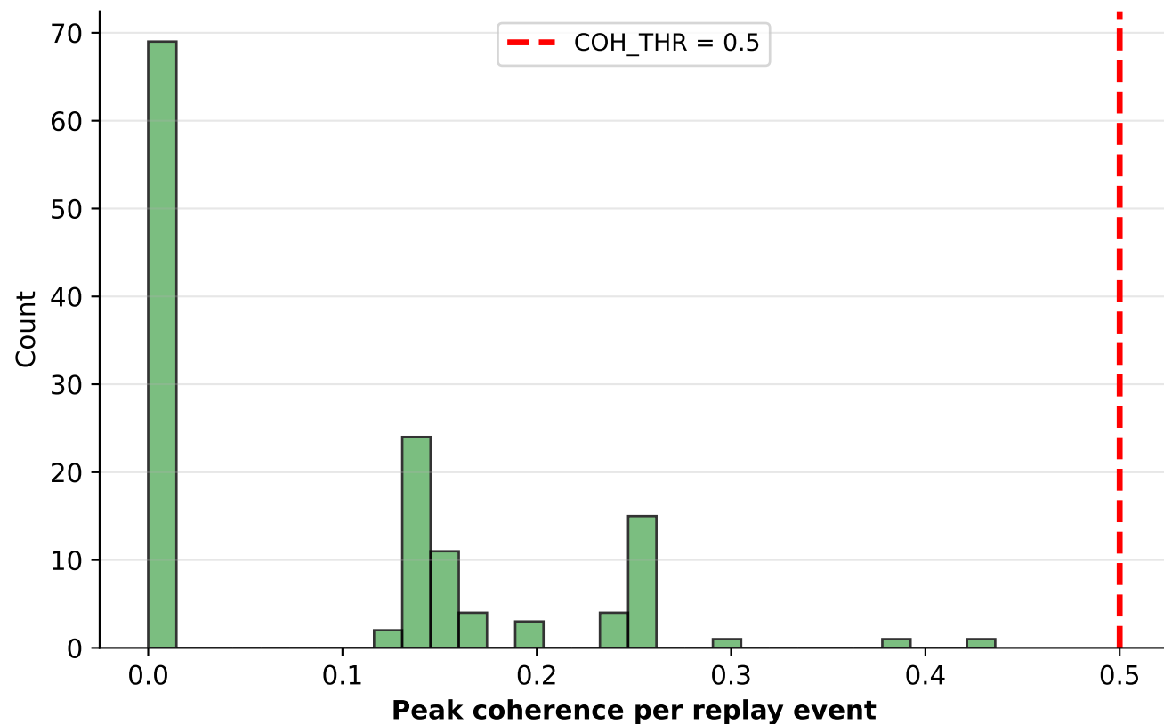
Peak Coherence Distribution max=0.436
