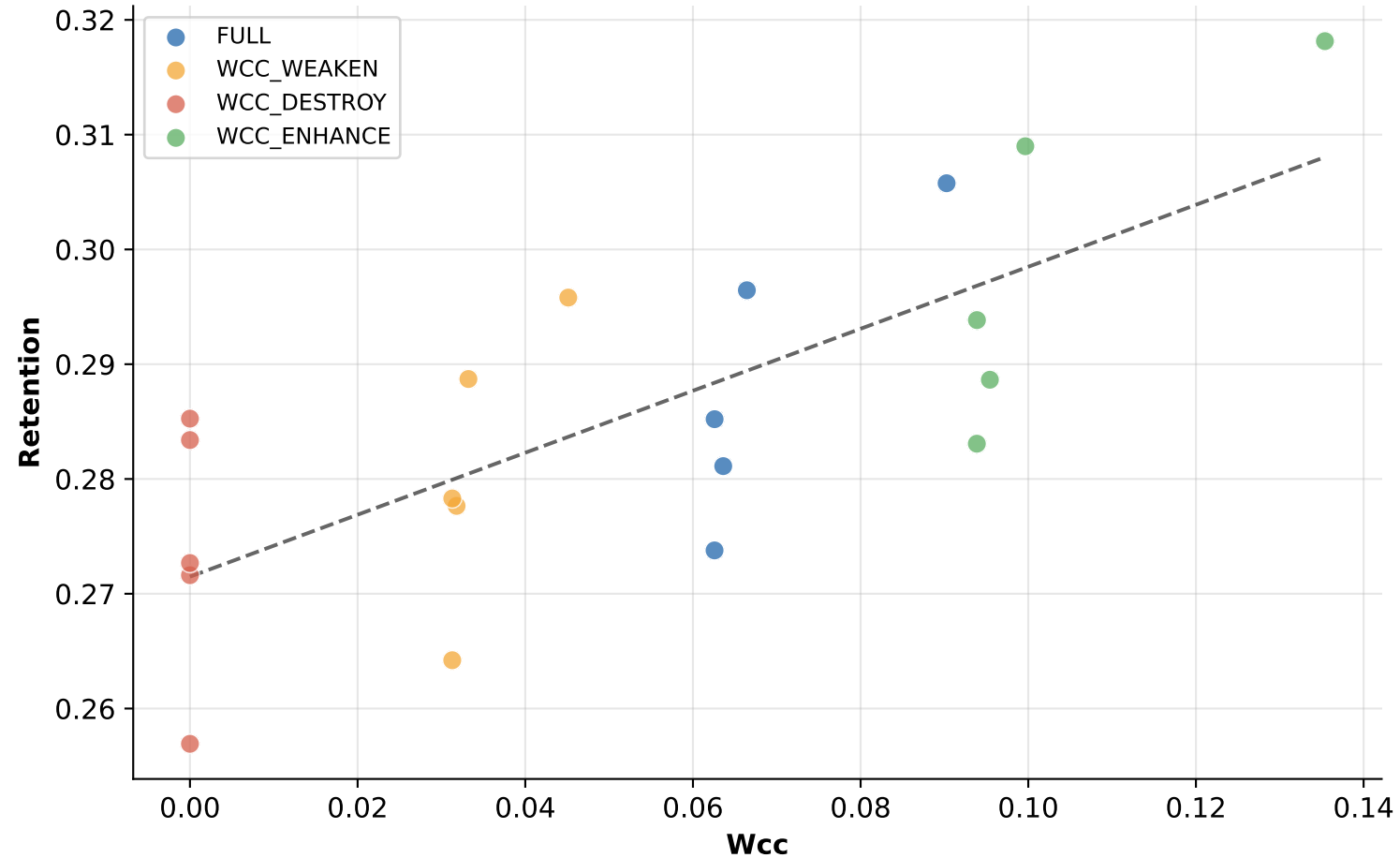
Retention vs Wcc (intervention sweep) r=+0.739 , p=1.98e-04 , R^2=0.546
