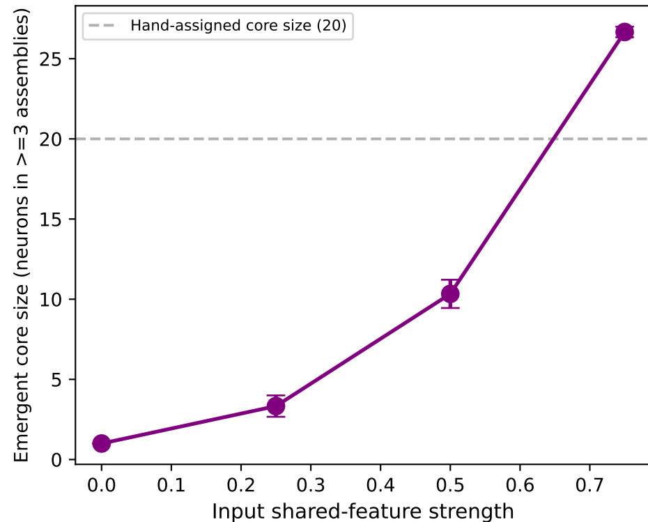
A. Does a schema core emerge from correlated inputs?
