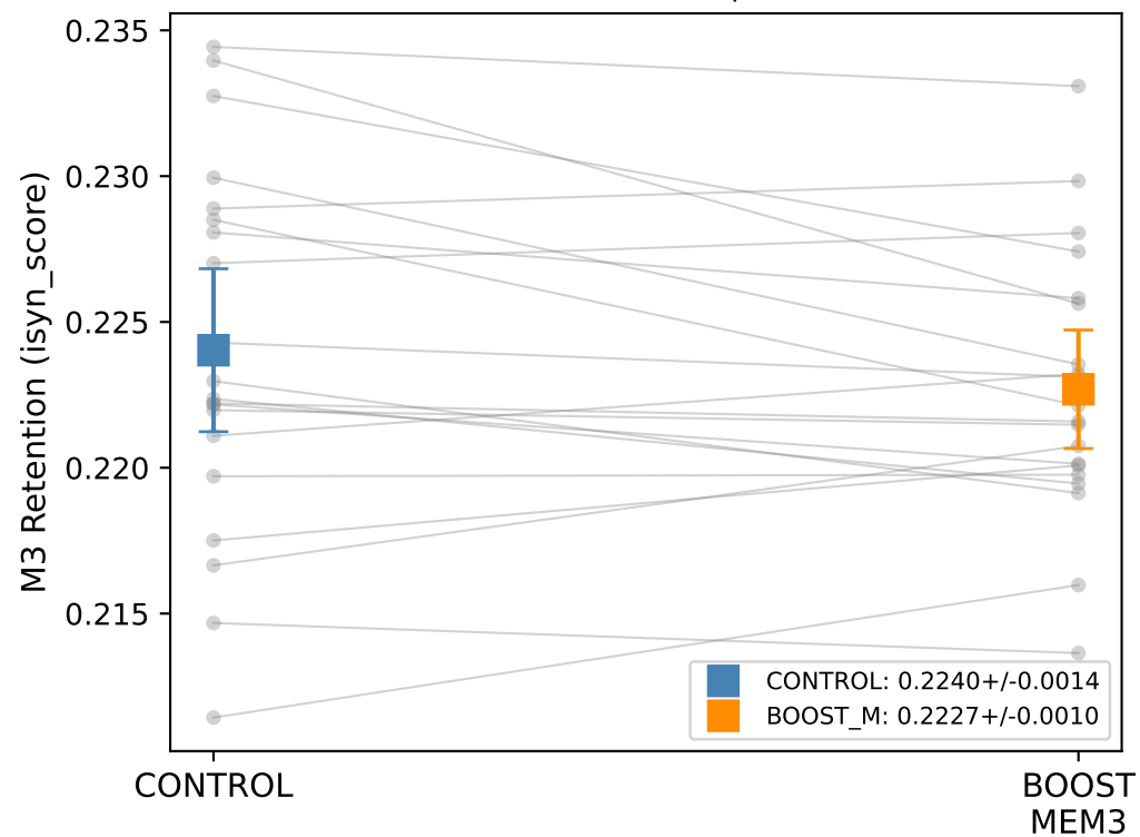
B. Boosting fails to rescue M3 ( n=20 seeds, t=1.72 , p=0.1024 )
