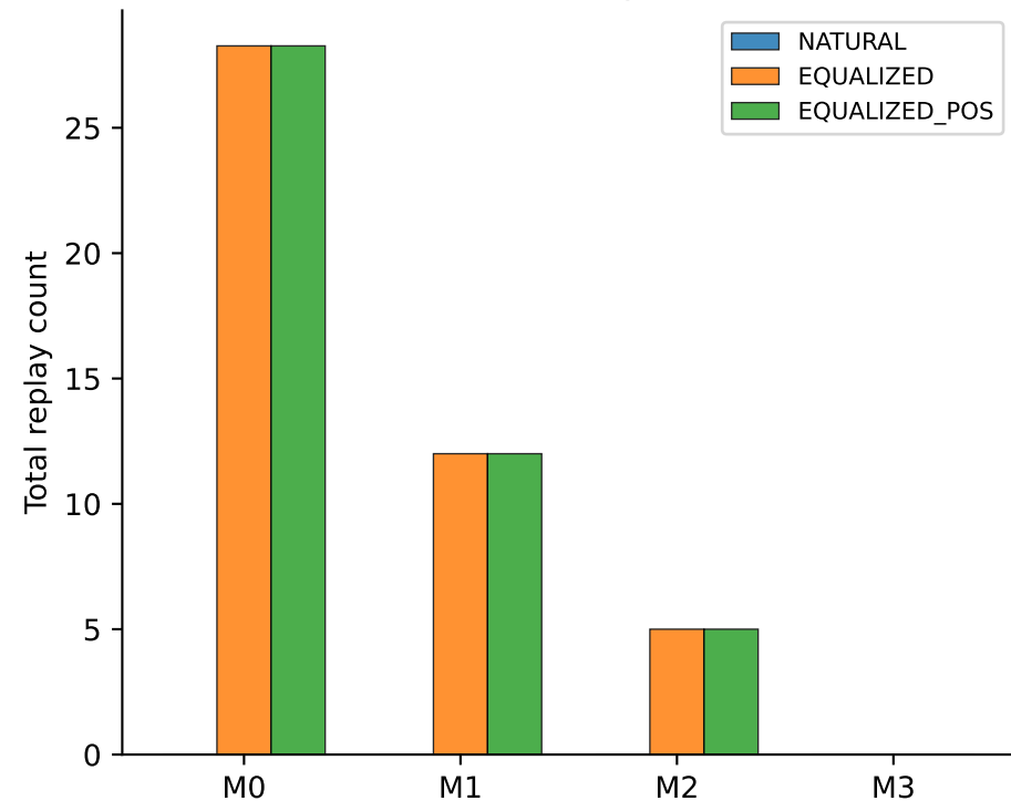
C. Replay allocation (verification of equalization)
