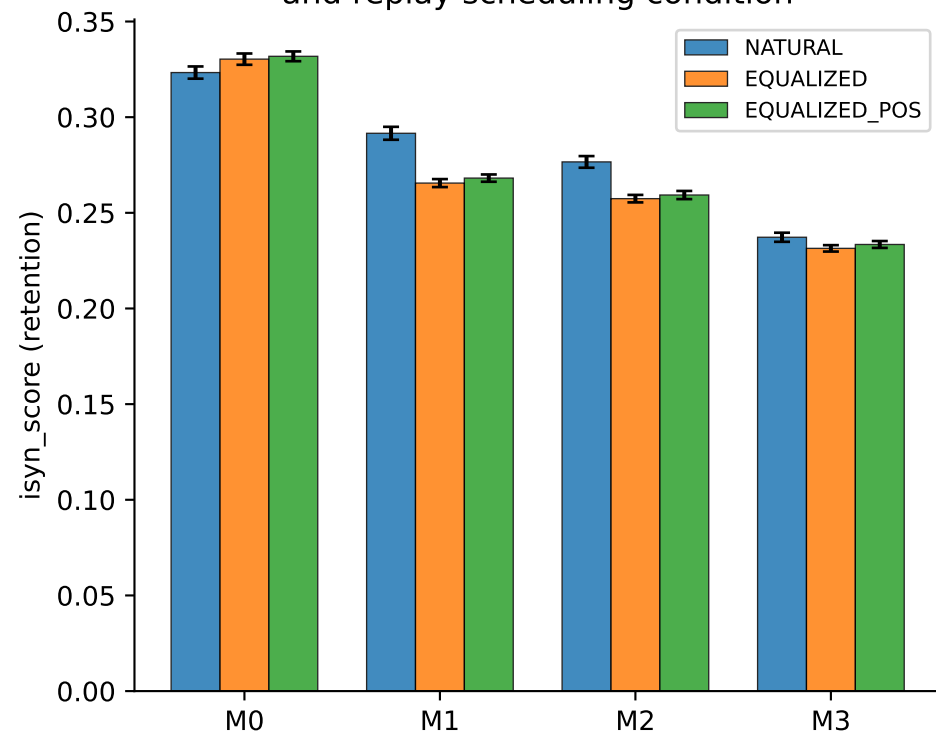
A. Retention by memory position and replay scheduling condition
