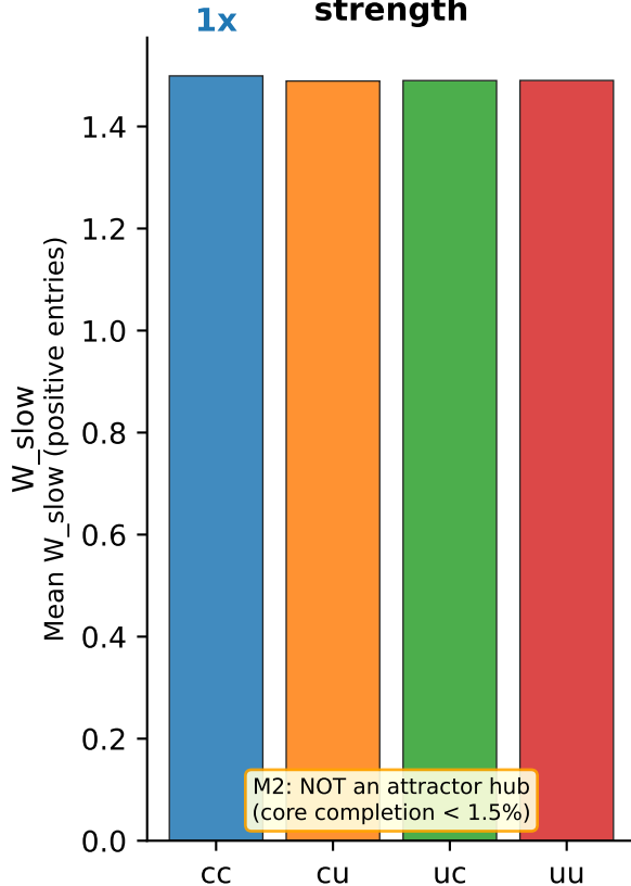
B. Block-level consolidation strength
