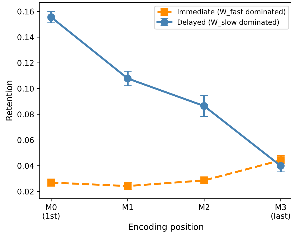
D. Serial position curves (4 memories, 10 seeds)
