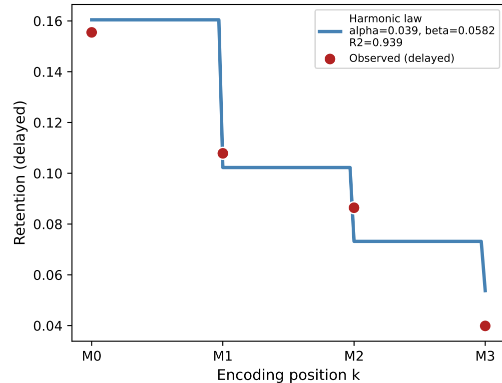
F. Position-to-consolidation law E[ret(k)] = \alpha + \beta \cdot (H(N) - H(k))
