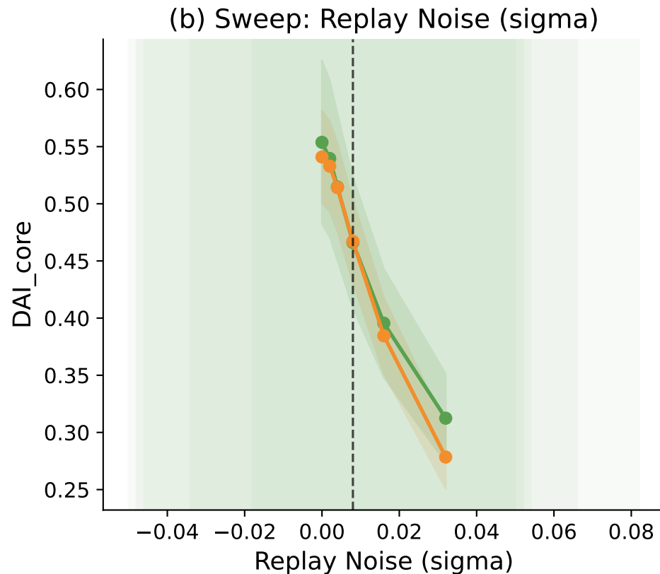
Figure 15: Robustness Parameter Sweep Natural > Hyper DAI_core across parameter ranges
