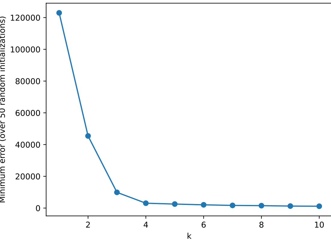
Minimum k-means error vs. k
