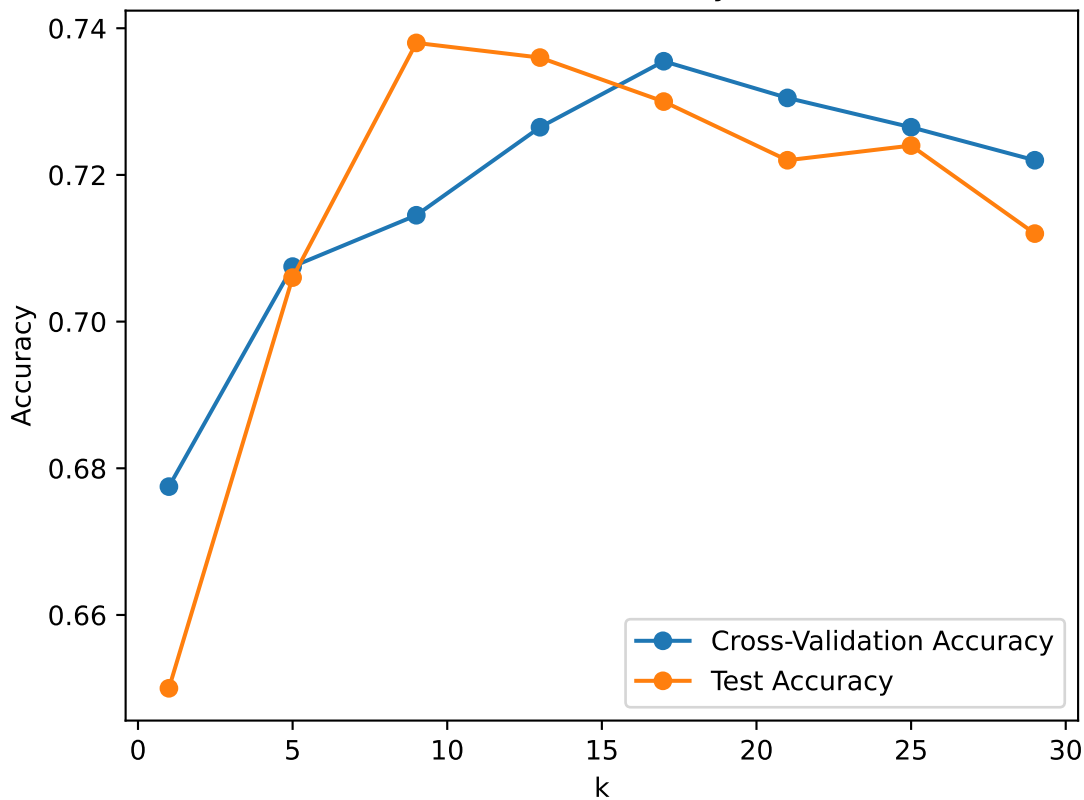
CV and Test Accuracy vs. k
