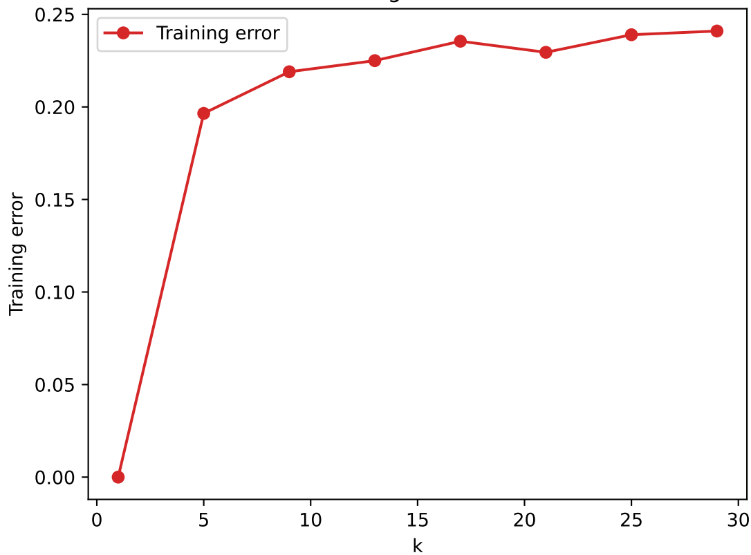
Training error vs. k
