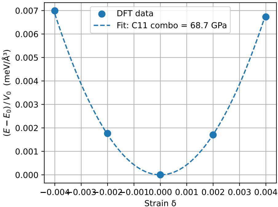
C11 strain set
