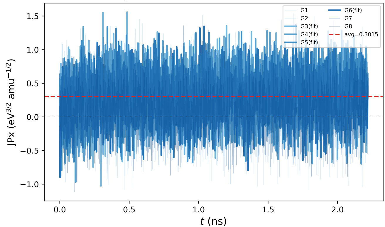
L_0500A avg(fit)=0.3015 Q=9.523e+08 W/m 2
