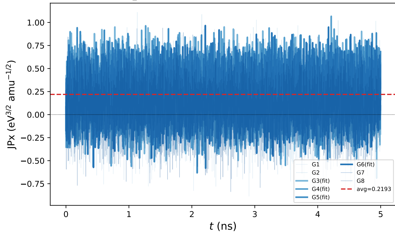
L_0250A avg(fit)=0.2193 Q=1.385e+09 W/m 2
