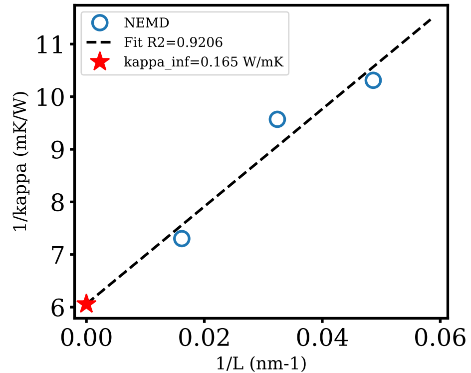
Finite-size correction
