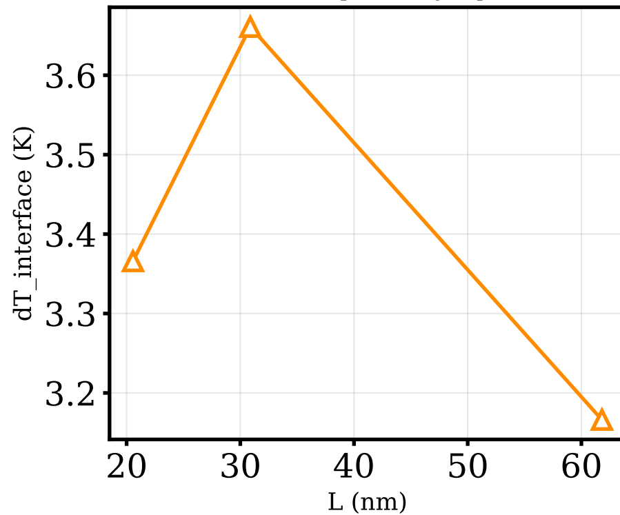
Interface Temperature Jump vs L
