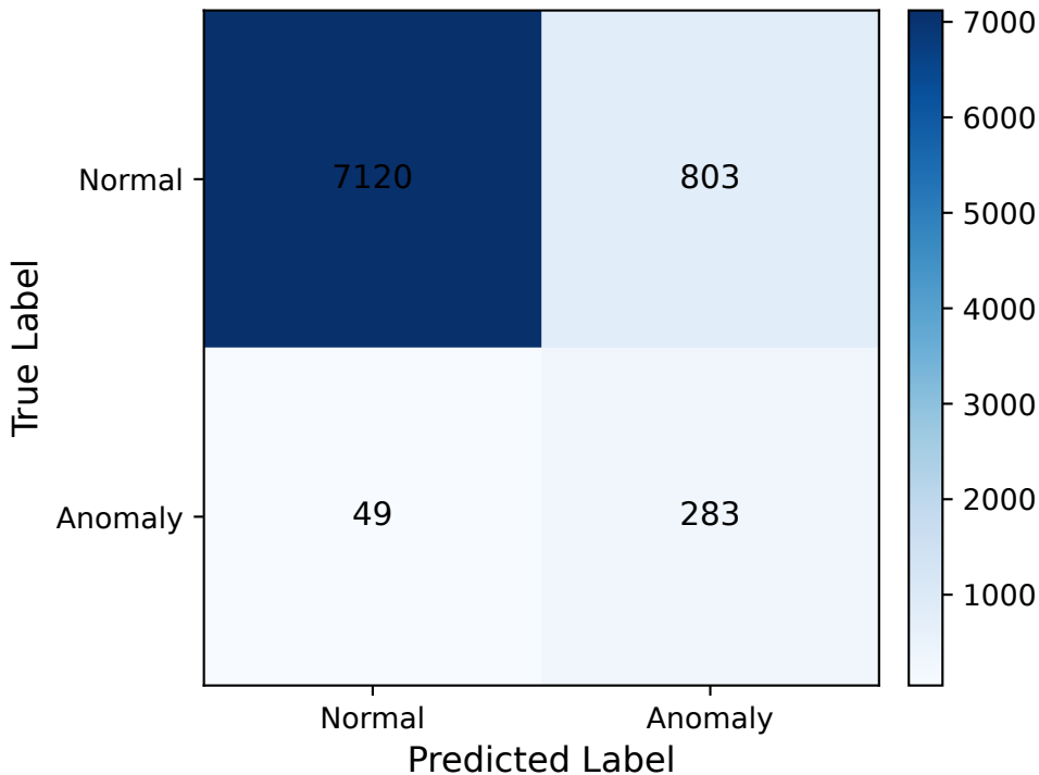
Confusion Matrix: Classical
