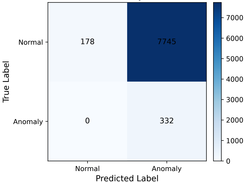
Confusion Matrix: Hybrid Quantum
