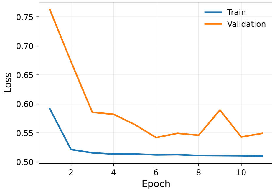
Reconstruction Loss
