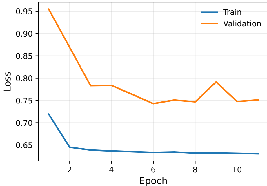
Total Loss
