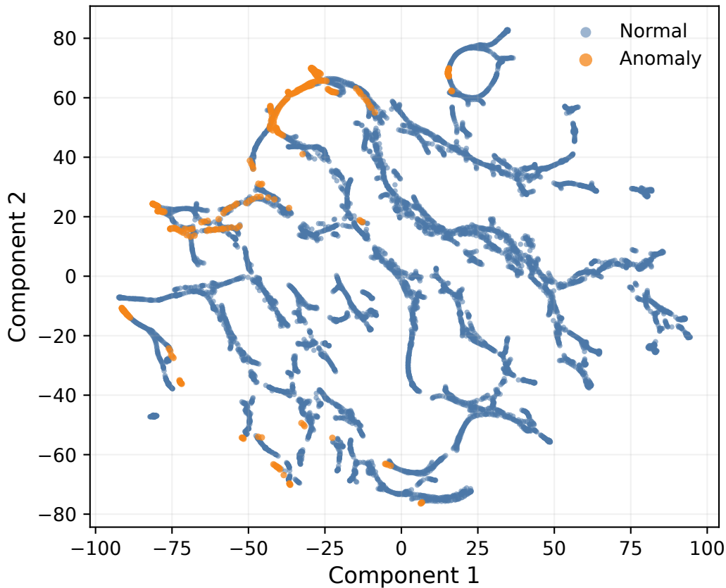
Latent t-SNE: Classical
