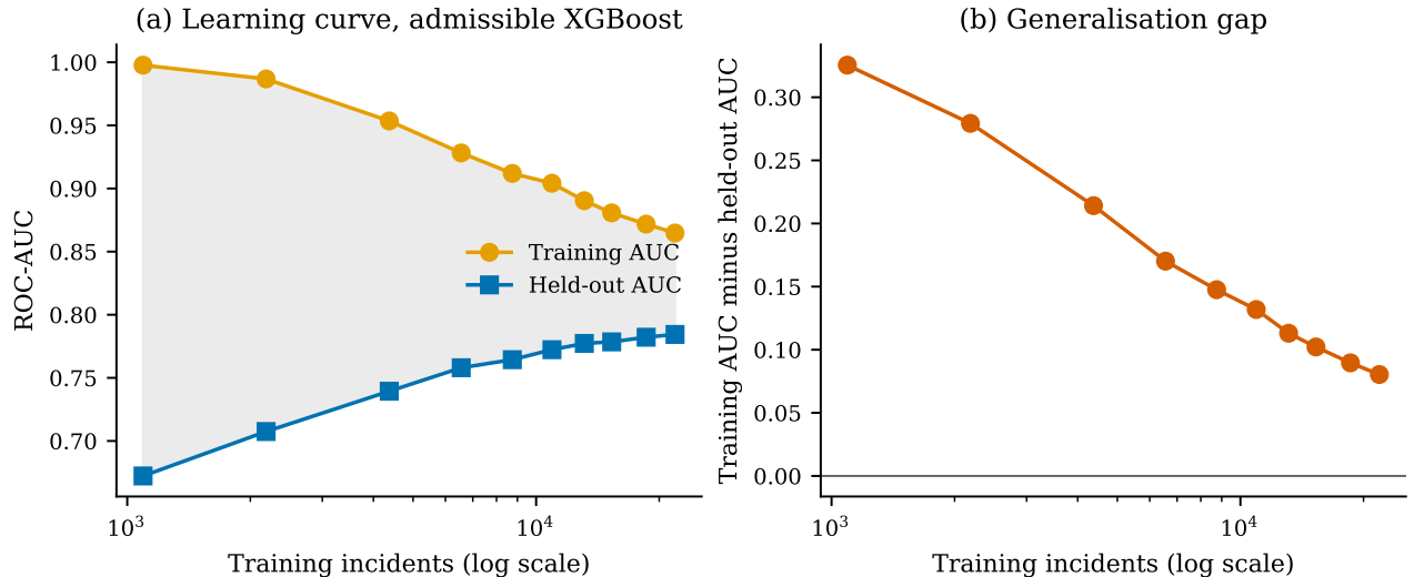
Fig. 8: Learning curve and generalisation gap. The two curves converge towards each other throughout and have not met, which is the signature of a model that is still data-limited rather than capacity-limited.
