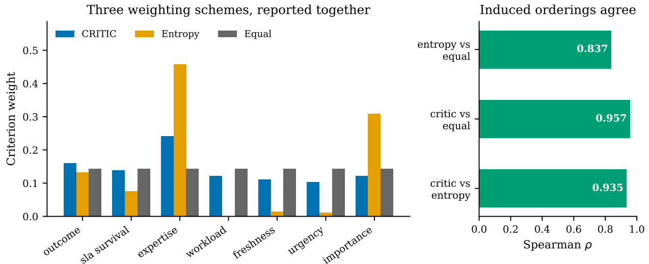
Fig. 14: The three weight vectors and the rank correlations between the orderings they induce.
