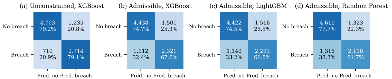
Fig. 4: Confusion matrices. Cell labels give counts and row-normalised percentages. Panel (a) is the model a practitioner would build without the protocol; panel (b) is the same learner under it.
