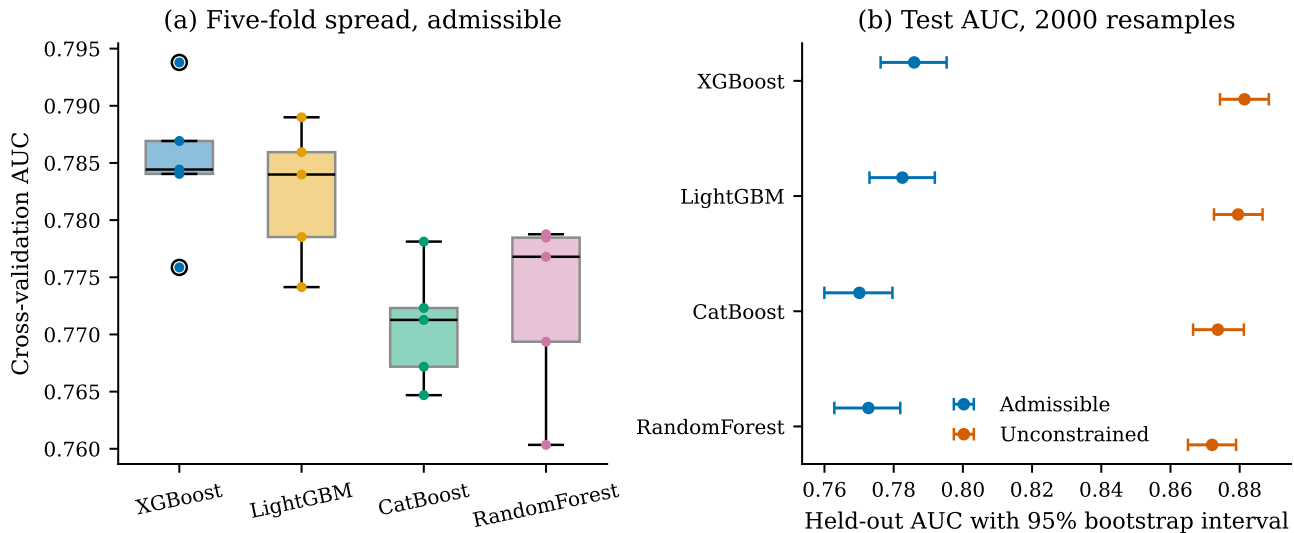
Fig. 9: Fold spread and bootstrap intervals. Panel (b) shows why the two configurations are distinguishable and the four learners within a configuration largely are not: the between-configuration separation is roughly ten times the width of any single interval.
