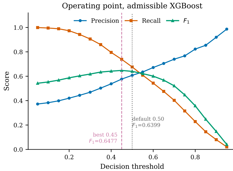
Fig. 10: Precision, recall and F_1 against the decision threshold. F_1 peaks at 0.45, not at the default 0.50.
