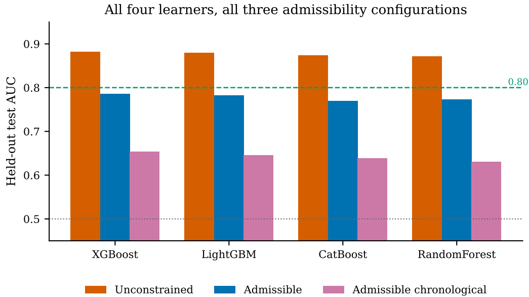
Fig. 3: Learner comparison across configurations. The correction is of the same size for every learner, which is what distinguishes a leakage effect from a modelling artifact.
