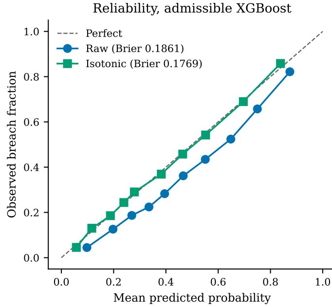
Fig. 11: Reliability of the admissible XGBoost model. Isotonic calibration reduces the Brier score from 0.1861 to 0.1769 while leaving AUC unchanged at 0.7859 against 0.7858, as a monotone transform must.
