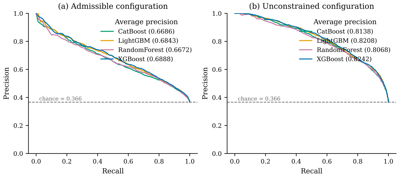
Fig. 6: Precision-recall curves. The dashed line is the chance level, which under precision-recall is the class prevalence 0.3664 rather than 0.5.
