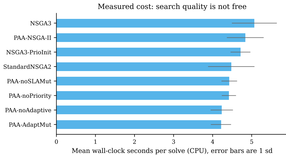
Fig. 18: Measured wall time per solve, 20 solves per variant, single CPU. Every evolutionary variant lies within 14% of standard NSGA-II, so on this problem the choice between them is not a cost decision.
