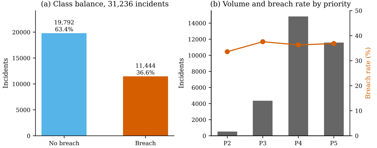
Fig. 1: Class balance and priority composition. The positive class is a 36.6% minority, which is imbalanced enough that accuracy alone would be misleading and is why precision, recall, the Matthews correlation coefficient and average precision are reported throughout.
