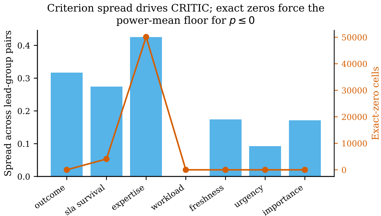
Fig. 13: Criterion distributions and the exact-zero counts that drive the degeneracy in Equation 12.
