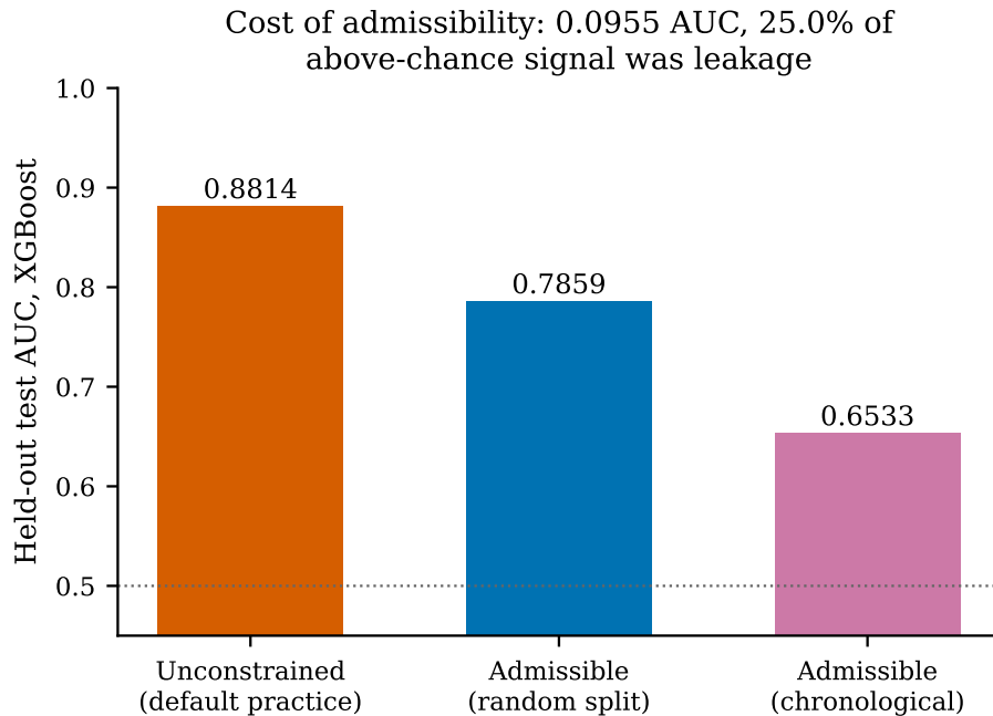
Fig. 2: Where the unconstrained model’s discrimination goes when each rule is applied.
