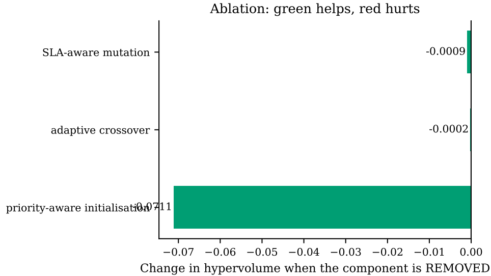
Fig. 16: Component ablation. Removing priority-aware initialisation costs 0.0711 hypervolume; removing either of the other two costs less than 0.001, which is inside run-to-run noise. Reporting the three as a bundle would have credited them equally.
