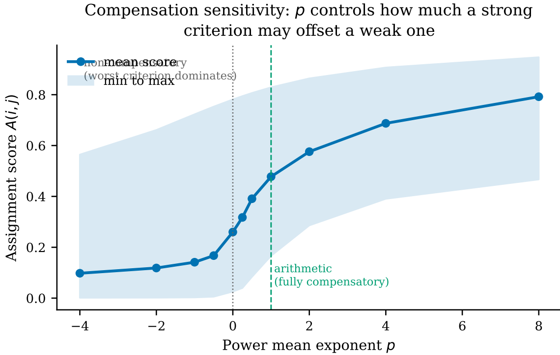
Fig. 15: Assignment score against the compensation exponent. The curve is monotone in p , as the power-mean inequality requires, which is a useful implementation check as well as a property.
