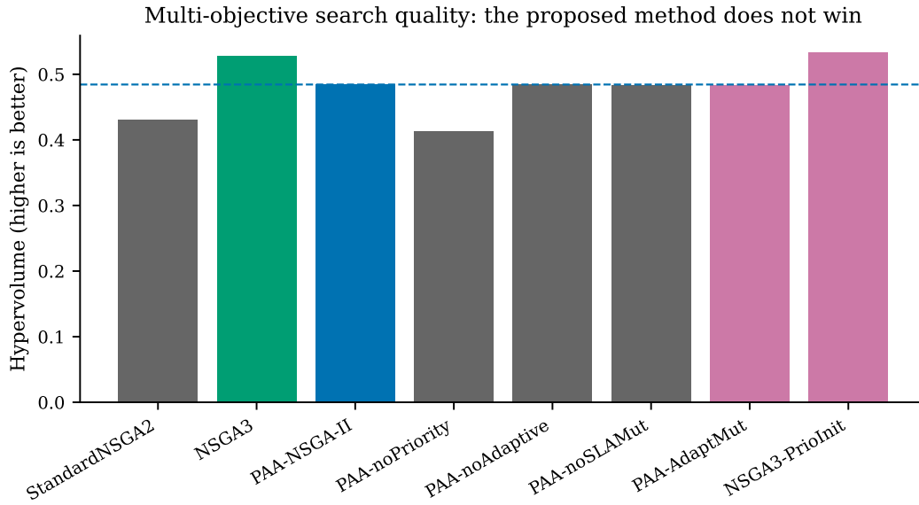
Fig. 17: Search quality across algorithm variants. The proposed method improves on its own base algorithm and is in turn outperformed by an off-the-shelf many-objective control.
