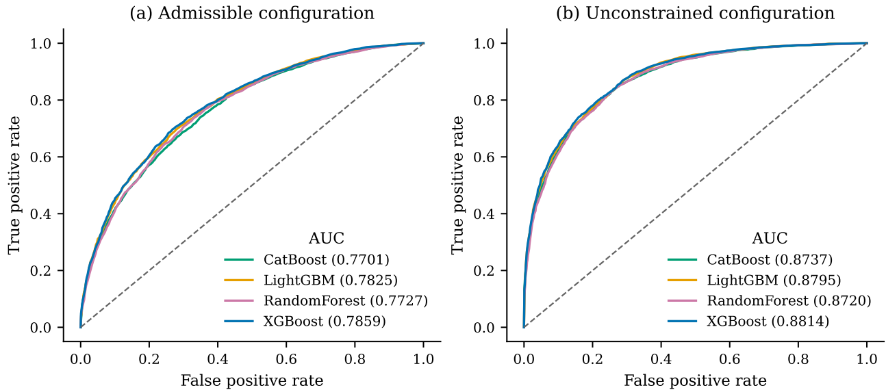
Fig. 5: ROC curves for all four learners under both configurations. The four curves are almost superimposed within each panel, which is the visual form of the result that the learner choice is not what drives performance here.
