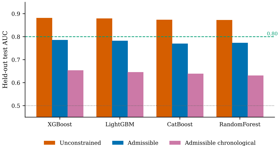
All four learners, all three admissibility configurations
