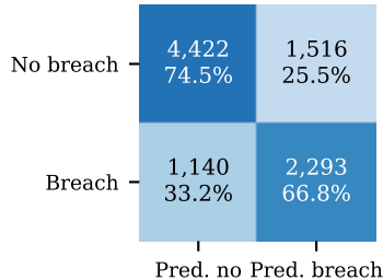
(c) Admissible, LightGBM
