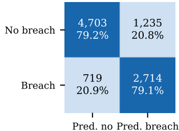
(a) Unconstrained, XGBoost
