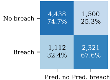
(b) Admissible, XGBoost
