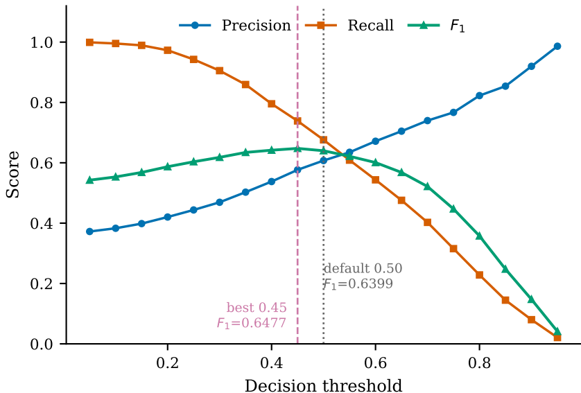
Operating point, admissible XGBoost
