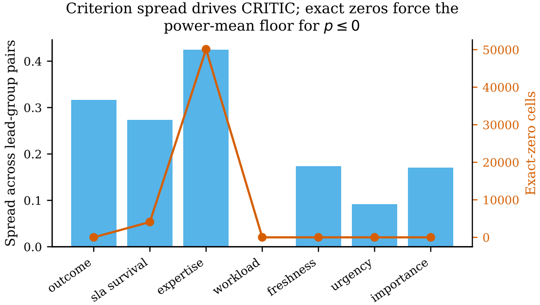
Figure 13: Criterion distributions and the exact-zero counts that drive the degeneracy in Equation 10.
