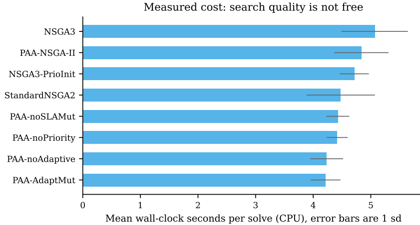
Figure 18: Measured wall time per solve, 20 solves per variant, single CPU. Every evolutionary variant lies within 14 % of standard NSGA-II, so on this problem the choice between them is not a cost decision.
