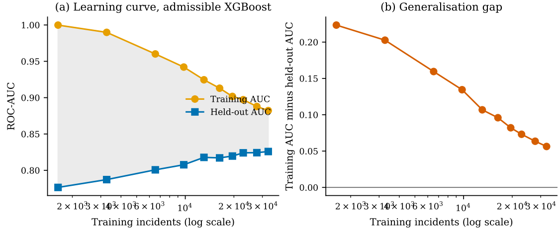
Figure 10: Learning curve and generalisation gap. The two curves converge towards each other throughout and have not met, which is the signature of a model that is still data-limited rather than capacity-limited.
