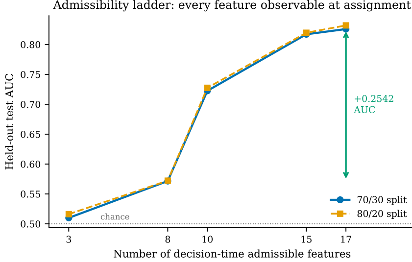
Figure 9: The admissible feature ladder under both split ratios. The two curves agree to within 0.0062 AUC at every rung, and the gain from eight attributes to seventeen agrees to within 0.0053. The cost of admissibility is tighter still, 0.0789 at 70/30 against 0.0793 at 80/20, so what the split ratio moves is where each rung sits rather than what the ladder or the correction is worth.
