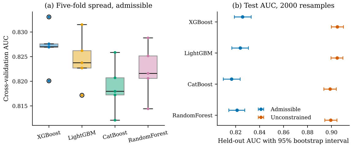
Figure 11: Fold spread and bootstrap intervals. Panel (b) shows why the two configurations are distinguishable and the four learners within a configuration largely are not: the between-configuration separation is roughly ten times the width of any single interval.
