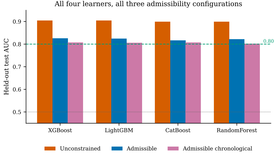
Figure 5: Learner comparison across configurations. The correction is of the same size for every learner, which is what distinguishes a leakage effect from a modelling artifact.
