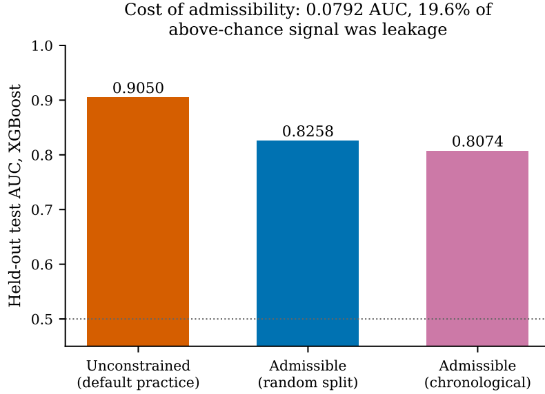
Figure 4: Where the unconstrained model’s discrimination goes when each rule is applied.
