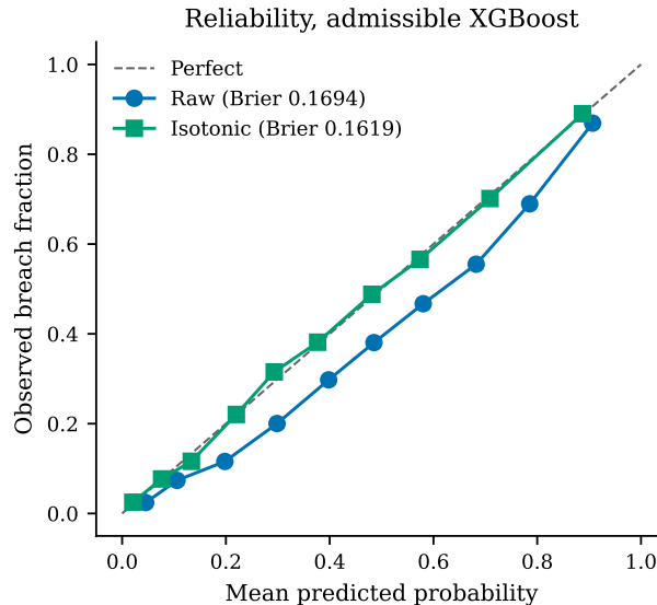
Figure 13: Reliability of the admissible XGBoost model. Isotonic calibration reduces the Brier score from 0.1694 to 0.1619 while leaving AUC essentially unchanged at 0.8258 against 0.8253, as a monotone transform must.
