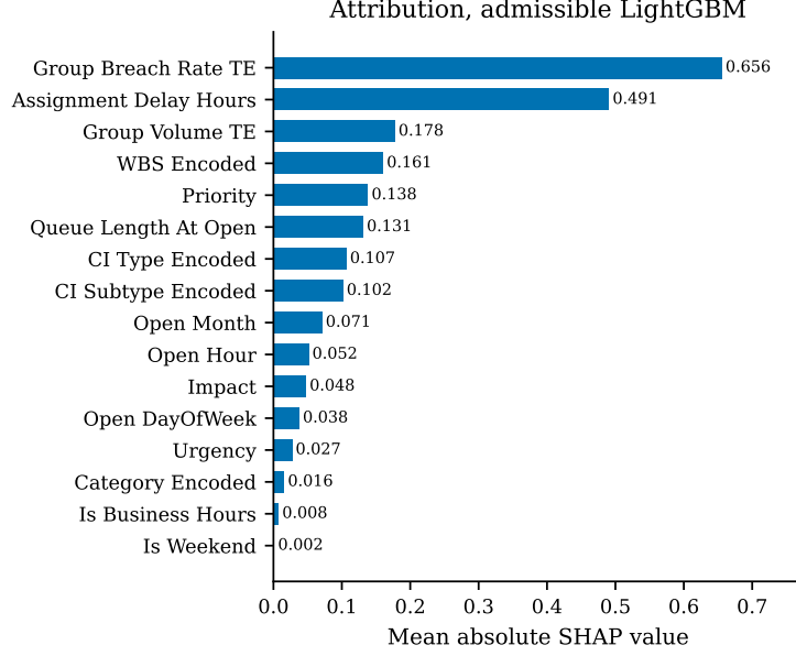
Figure 14: Mean absolute SHAP attribution, admissible LightGBM. LightGBM is used here rather than XGBoost because shap 0.45.1 cannot parse the model JSON emitted by XGBoost 3.2.0; the two learners differ by only a small margin in test AUC on this feature set, so the attribution is representative of the admissible model reported elsewhere. Alert status contributes exactly zero and is retained in the table for completeness, because an attribute that survives the admissibility rules and then turns out to be uninformative is a different finding from one that was excluded.
