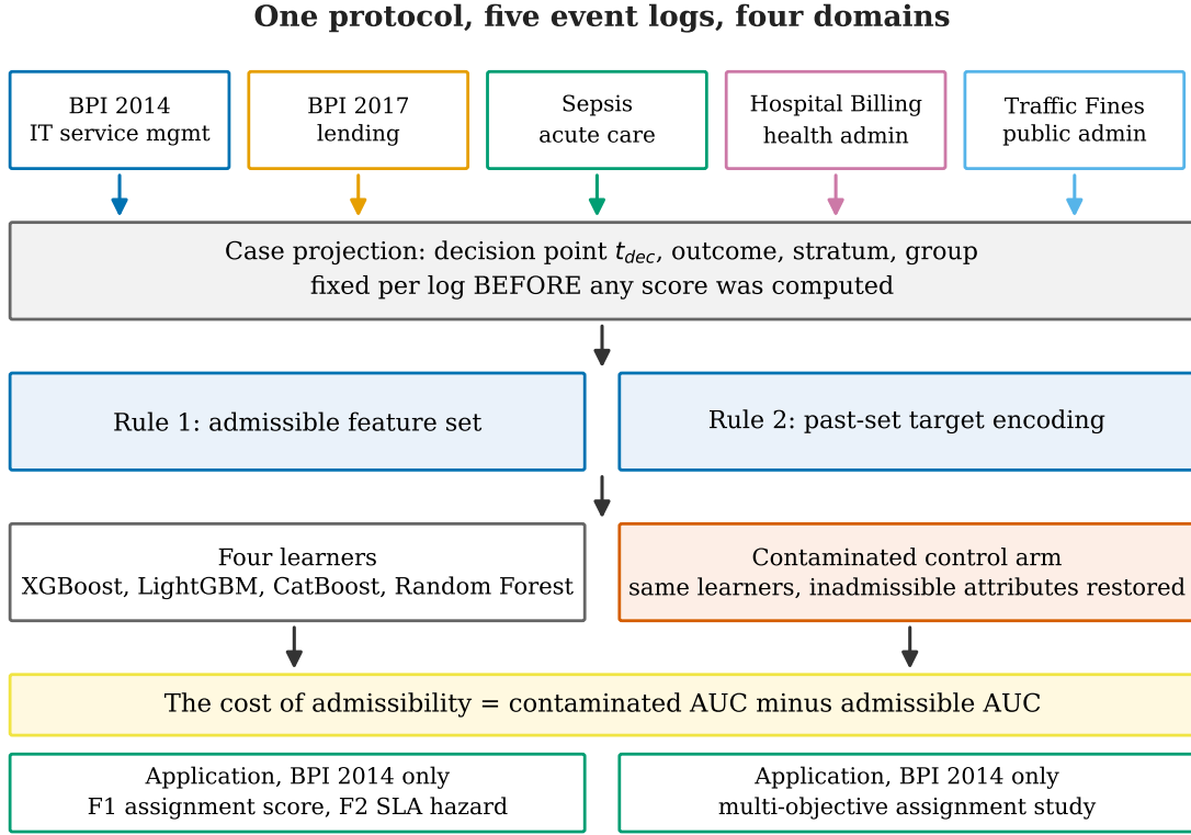
Figure 3: The apparatus end to end. Five event logs enter one code path; the admissibility filter of Figure 2 splits each into an unconstrained arm and an admissible arm, and the gap between what the two arms score is the measurement. The four learners are held fixed across arms by design, so a difference between arms is a property of the constraint and not of the model. The scoring formulations and the assignment layer on the right run on BPI 2014 only, and are what an admissible model is then used for.
