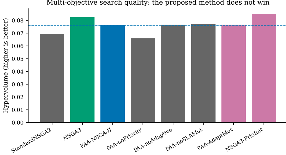
Figure 19: Search quality across algorithm variants. The proposed method improves on its own base algorithm and is in turn outperformed by an off-the-shelf many-objective control.
