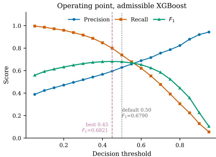
Figure 12: Precision, recall and F_1 against the decision threshold. F_1 peaks at 0.45, not at the default 0.50.
