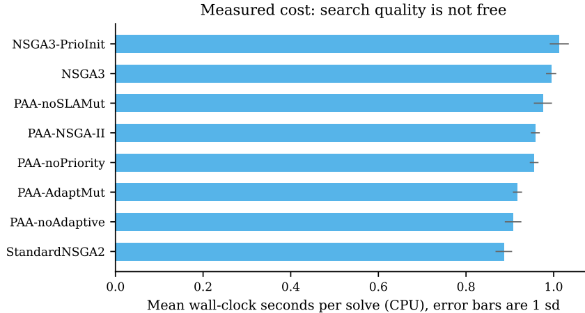
Figure 20: Measured wall time per solve, 20 solves per variant, single CPU. Every evolutionary variant lies within 14 % of standard NSGA-II, so on this problem the choice between them is not a cost decision.
