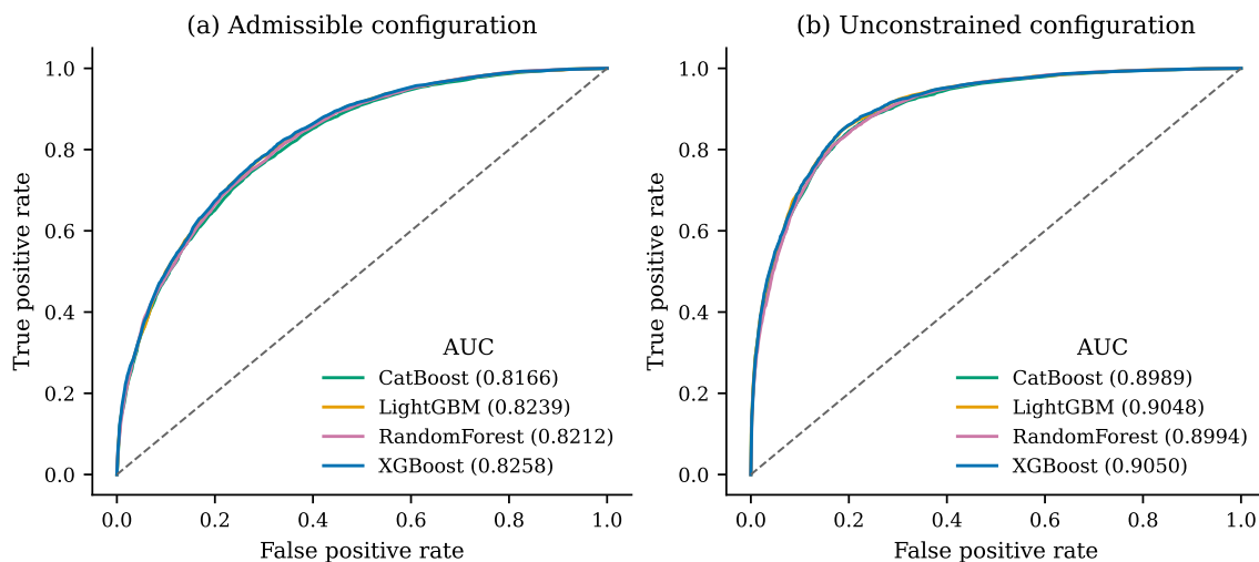
Figure 7: ROC curves for all four learners under both configurations. The four curves are almost superimposed within each panel, which is the visual form of the result that the learner choice is not what drives performance here.
