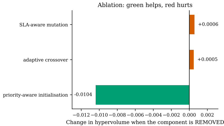
Figure 18: Component ablation. Removing priority-aware initialisation costs 0.0104 hypervolume; removing either of the other two changes it by less than 0.001 and in the opposite direction, which is inside run-to-run noise. Reporting the three as a bundle would have credited them equally.
