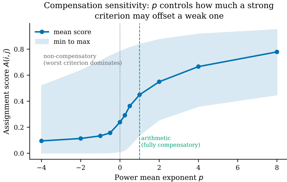
Figure 17: Assignment score against the compensation exponent. The curve is monotone in p , as the power-mean inequality requires, which is a useful implementation check as well as a property.
