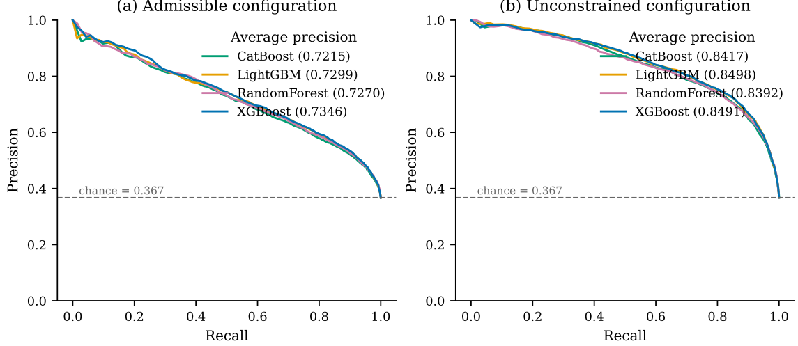
Figure 8: Precision-recall curves. The dashed line is the chance level, which under precision-recall is the class prevalence 0.3673 rather than 0.5.
