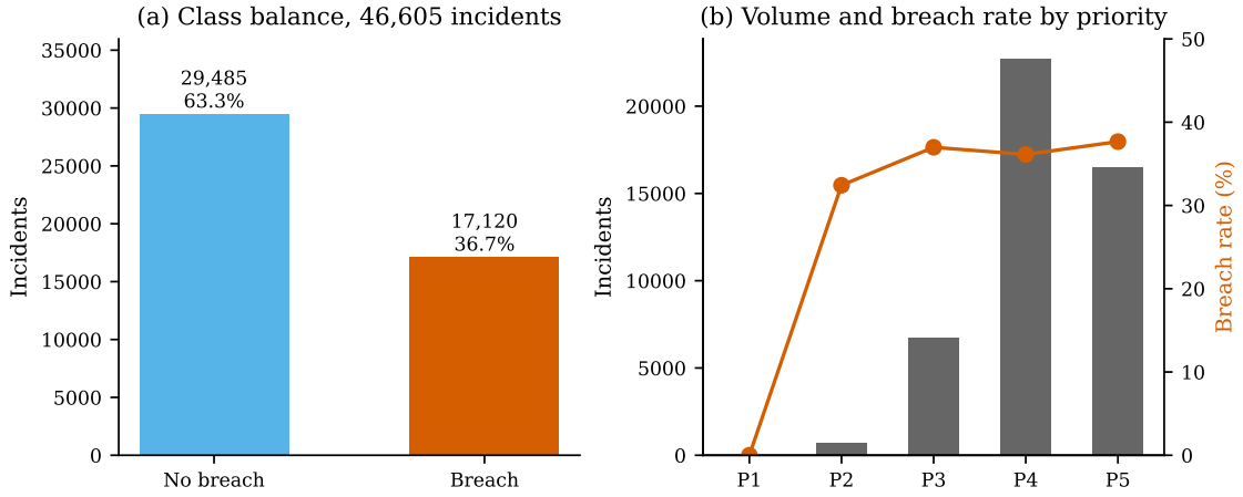
Figure 1: Class balance and priority composition. The positive class is a 36.7% minority, which is imbalanced enough that accuracy alone would be misleading and is why precision, recall, the Matthews correlation coefficient and average precision are reported throughout.
