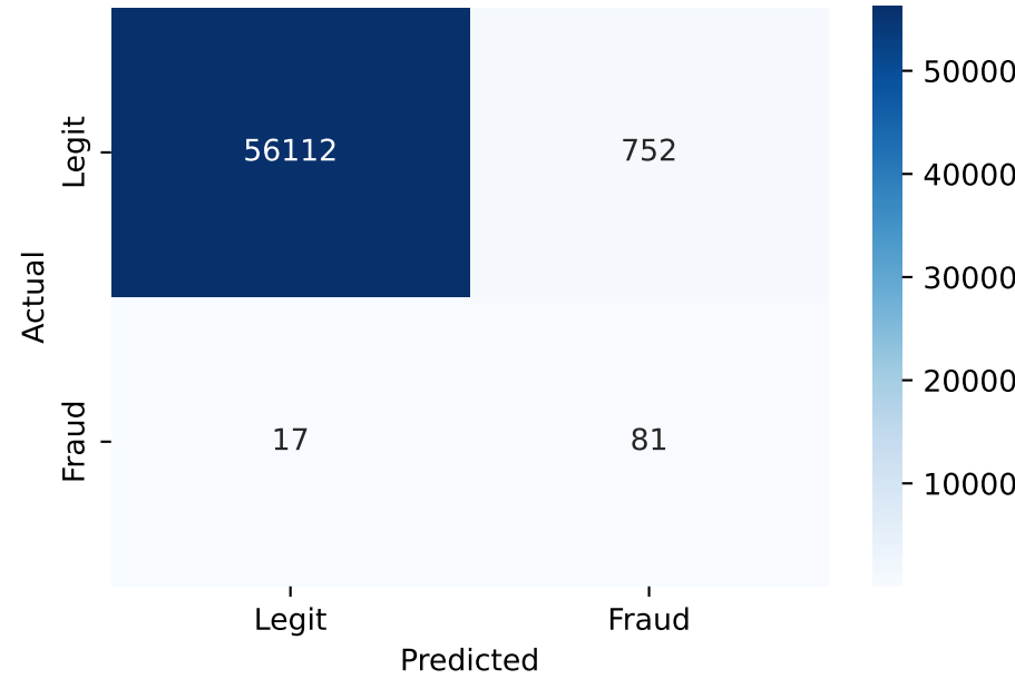
Decision Tree
