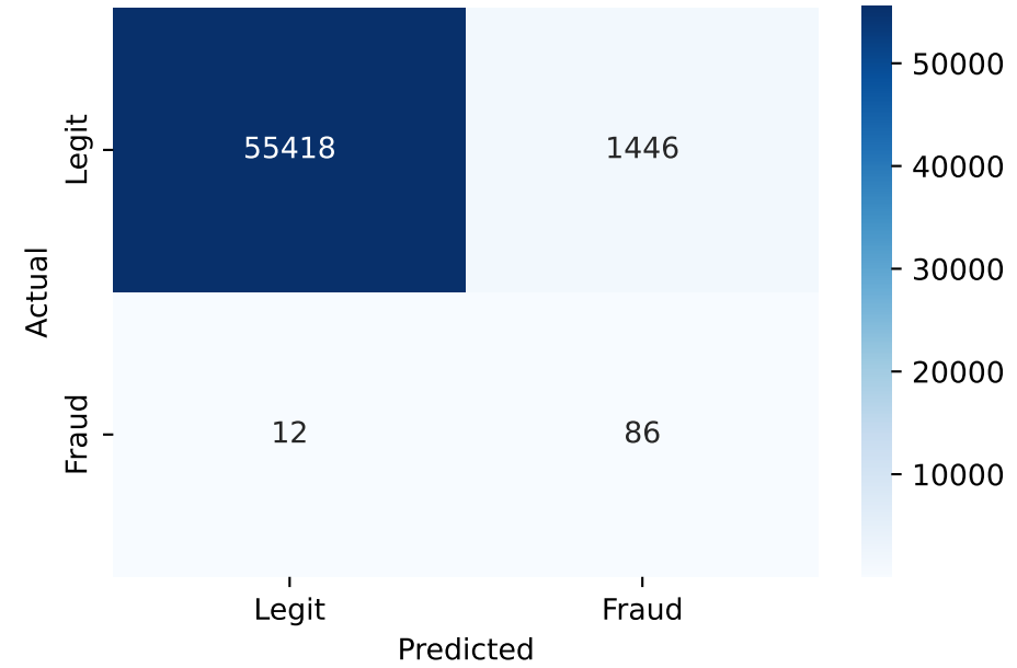
Naive Bayes
