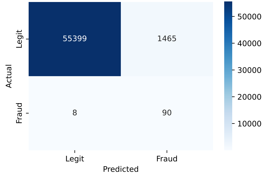
Logistic Regression
