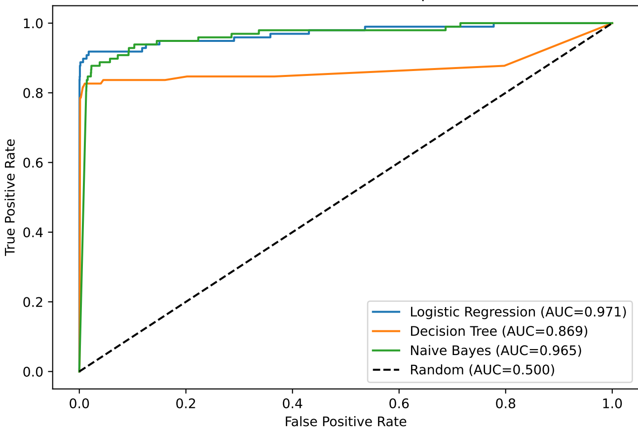
ROC Curves — Model Comparison
