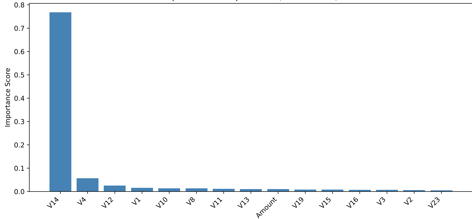
Top 15 Feature Importances (Decision Tree)
