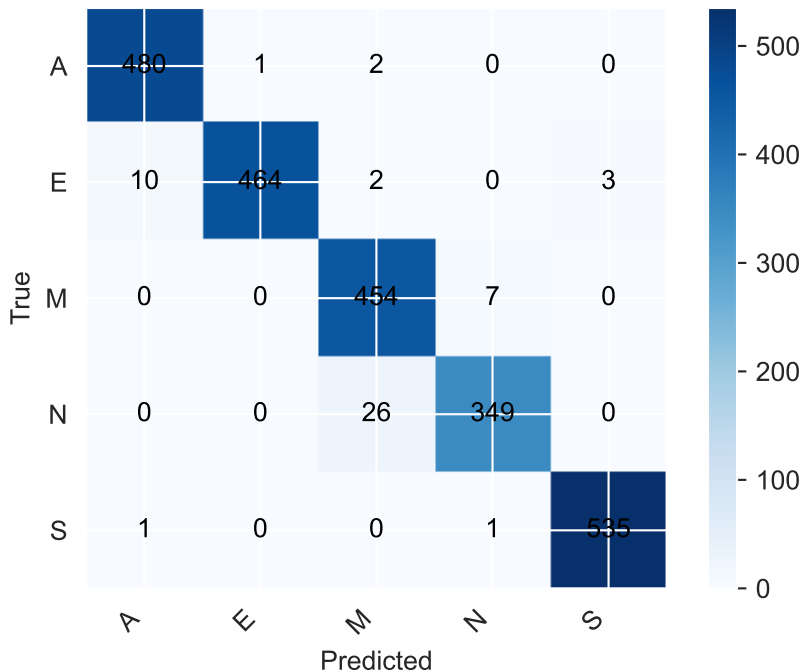
Ambiguous Letters - Ensemble
