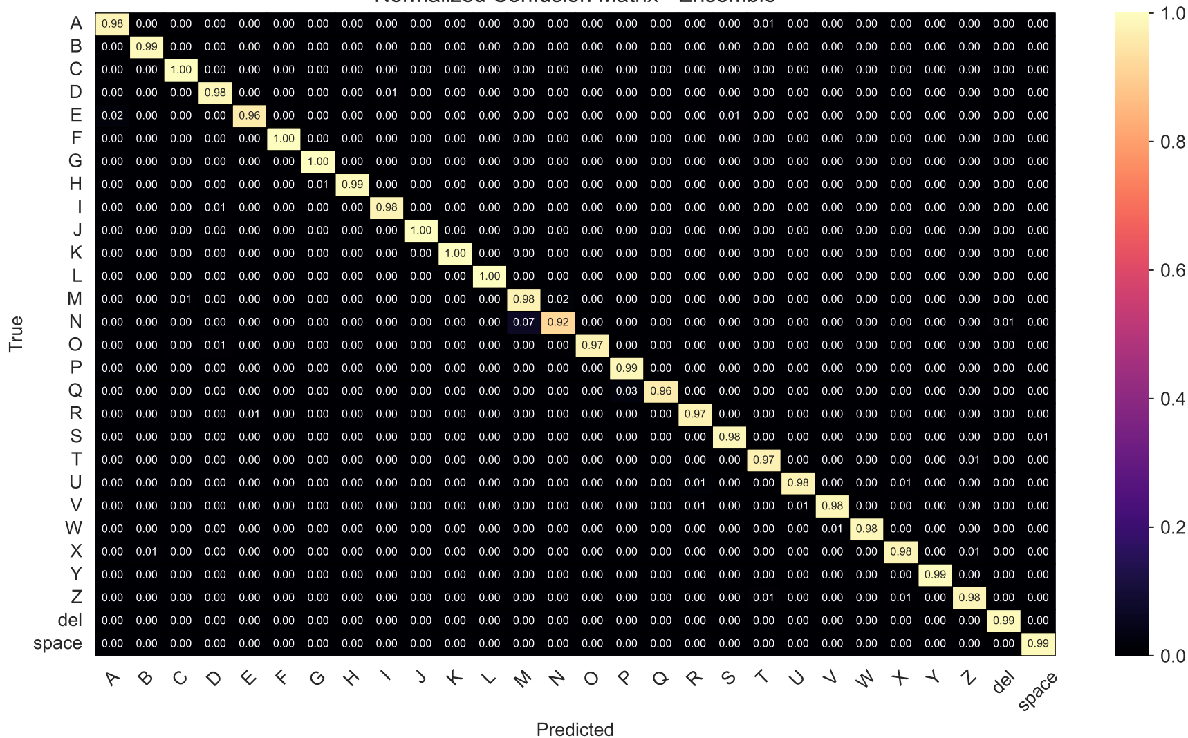
Normalized Confusion Matrix - Ensemble
