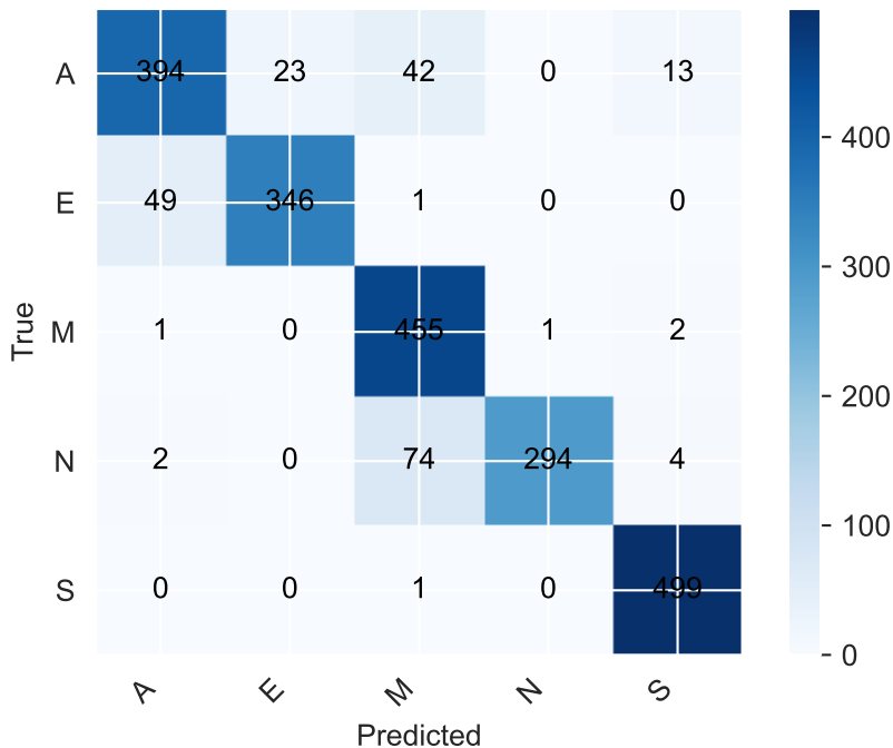
Ambiguous Letters - Custom CNN
