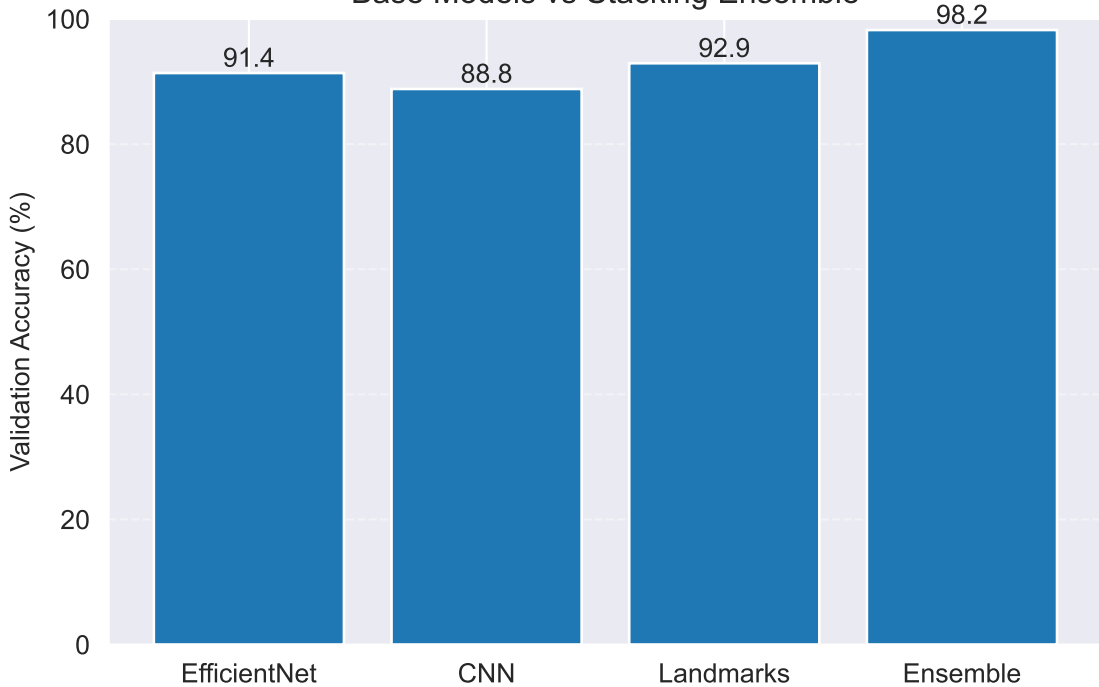
Base Models vs Stacking Ensemble
