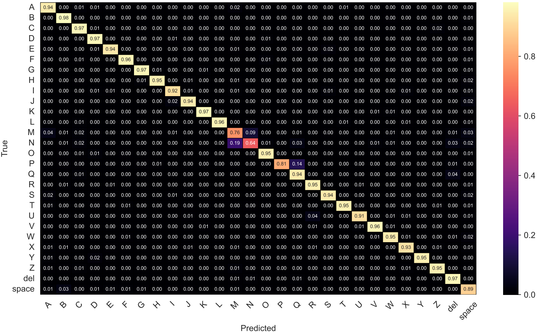
Normalized Confusion Matrix - Model C (Geometric)
