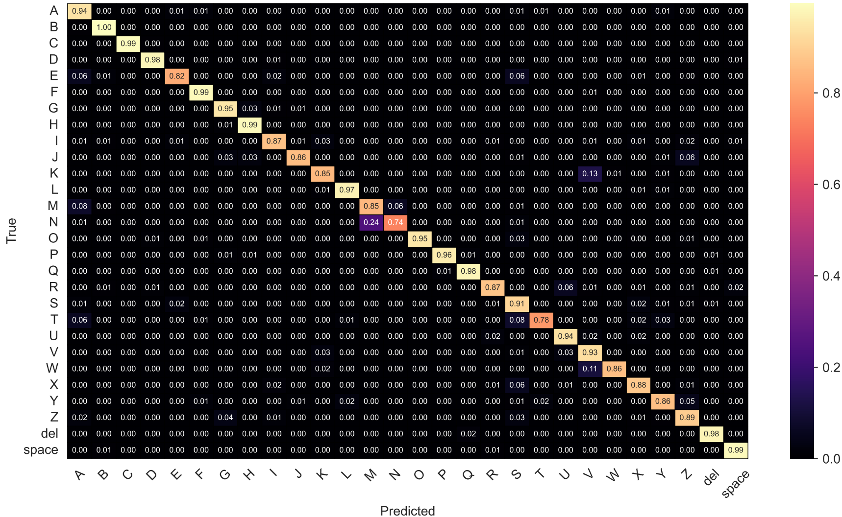
Normalized Confusion Matrix - Model E (EfficientNet)
