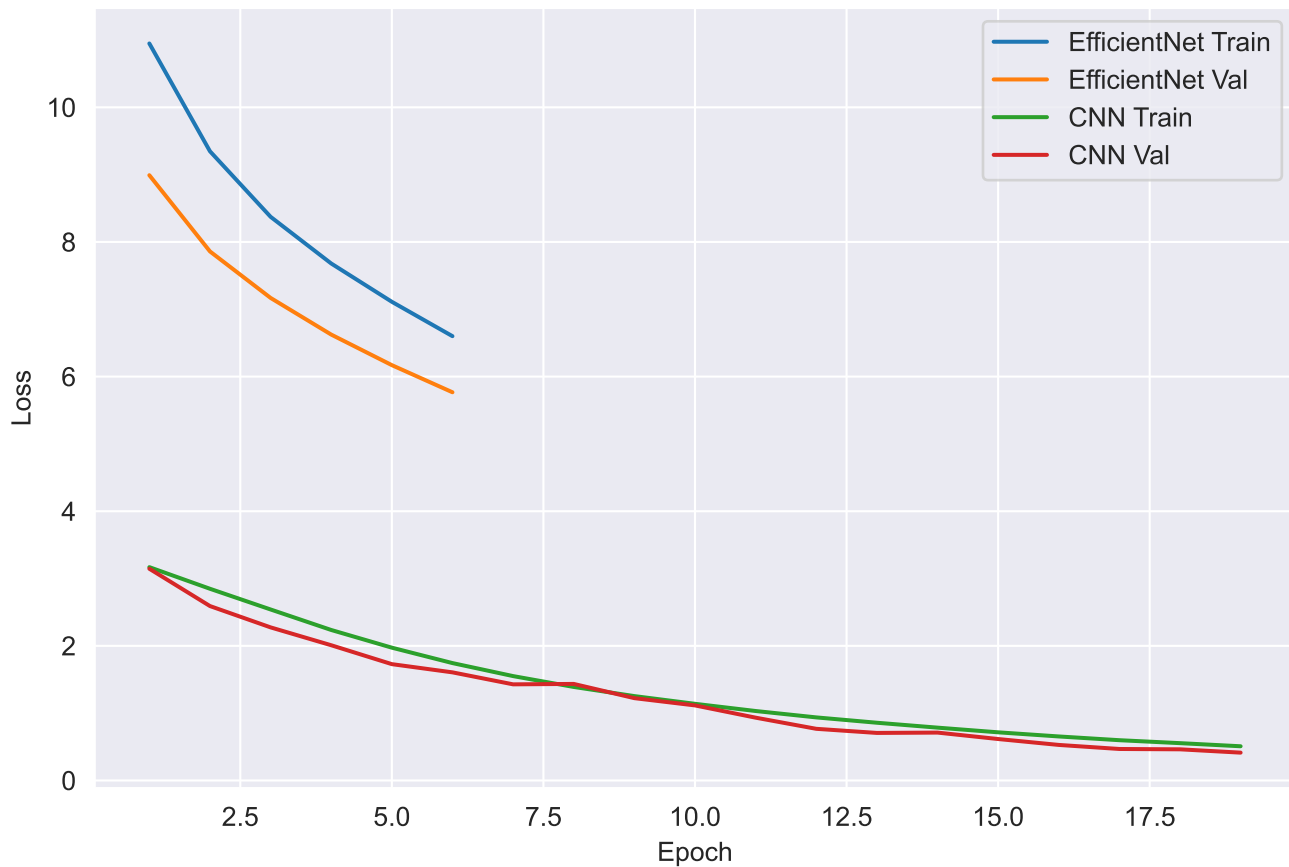
Learning Curves: EfficientNet vs CNN
