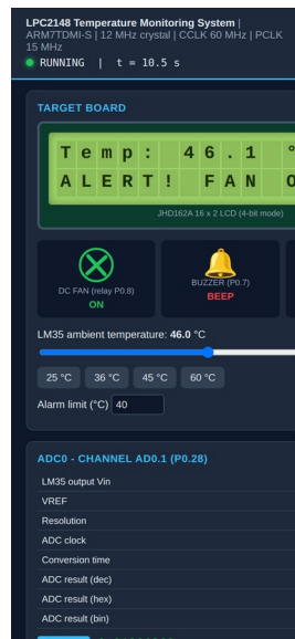
Fig. 9 - The simulator adapts to a 390 px wide phone screen.
