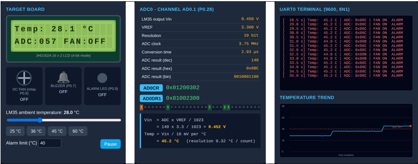
Fig. 7 - Left to right: LCD with fan / buzzer / LED status, ADC0 channel AD0.1 registers with the conversion formula, and the UART0 log with the trend graph.
