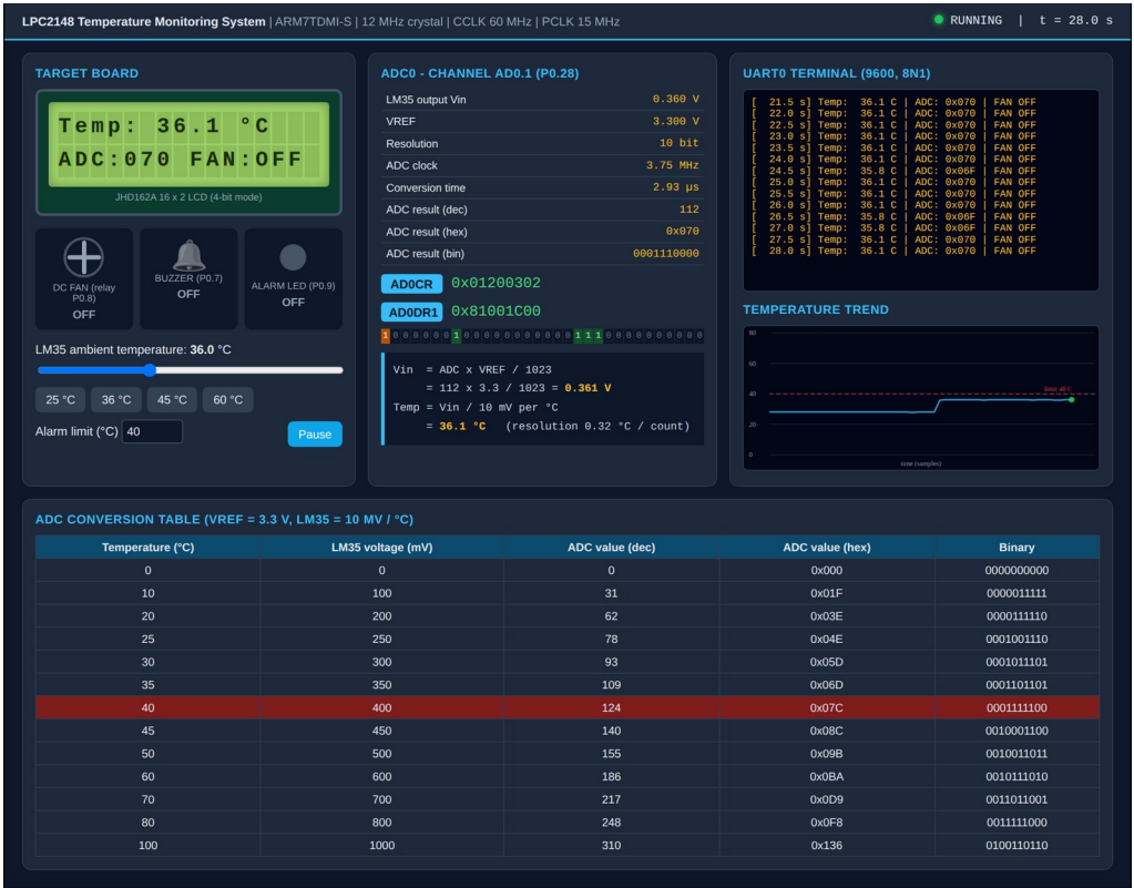
Fig. 2 - The UART log turns yellow near the limit but the fan is still OFF because 36 °C is below 40 °C.
