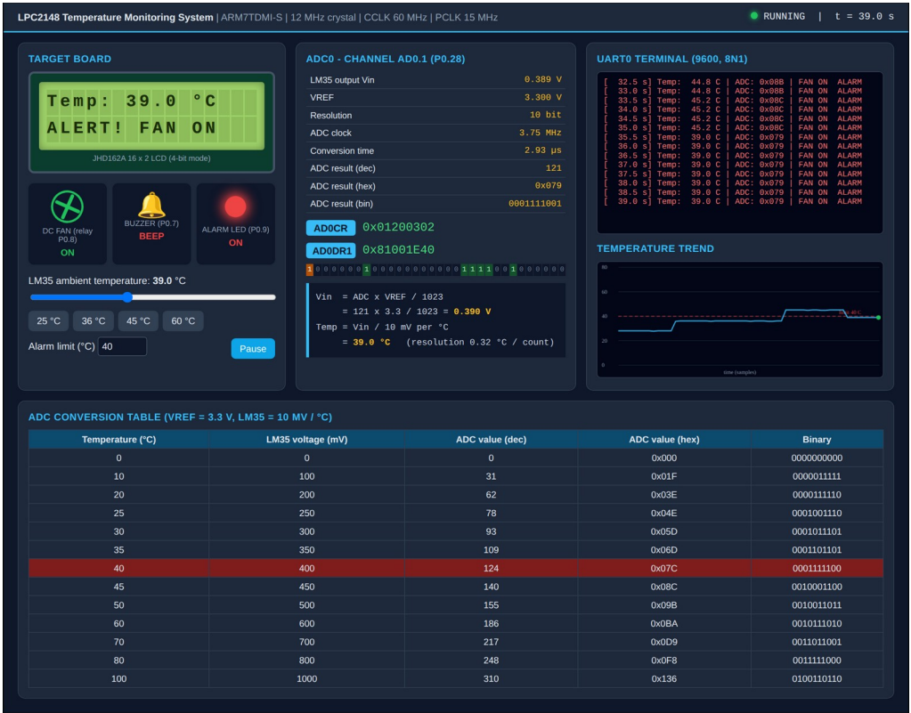
Fig. 4 - The temperature has dropped to 39 °C but the fan stays ON until it falls to 38 °C or below.
