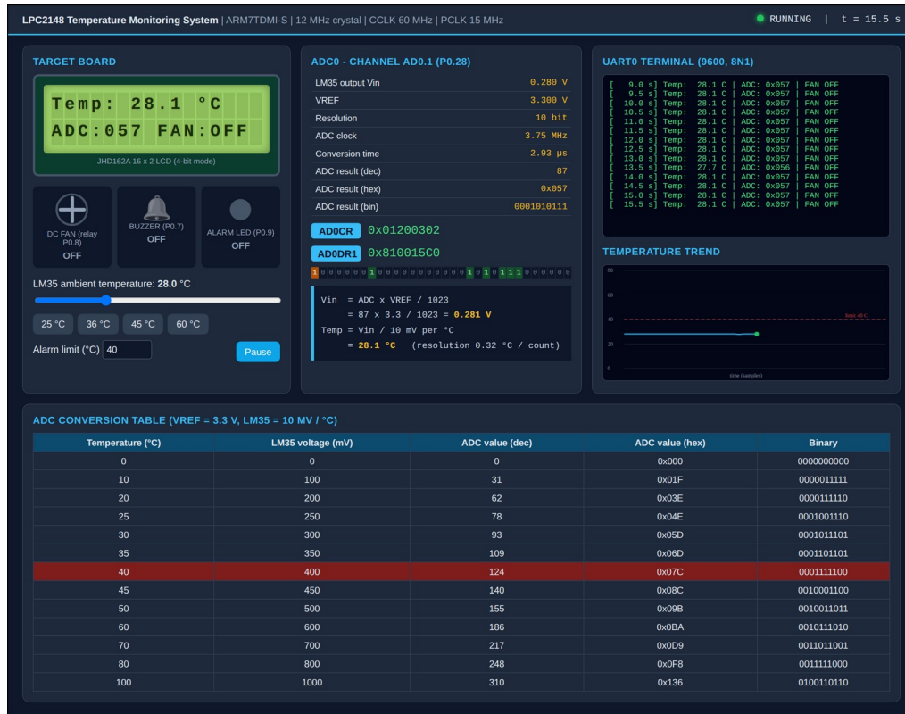
Fig. 1 - LCD shows Temp: 28.1 °C and ADC:057; the fan, buzzer and alarm LED are OFF; AD0DR1 shows DONE = 1.
