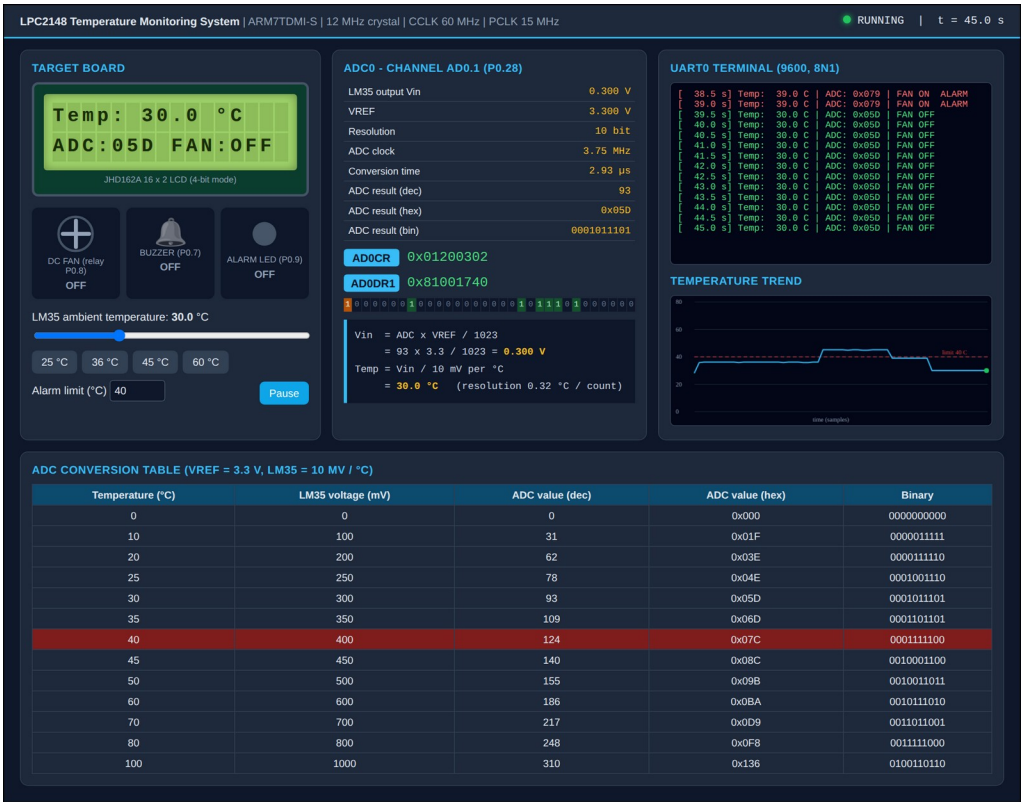
Fig. 5 - After cooling, the fan, buzzer and LED are switched OFF and the trend graph falls below the limit line.
