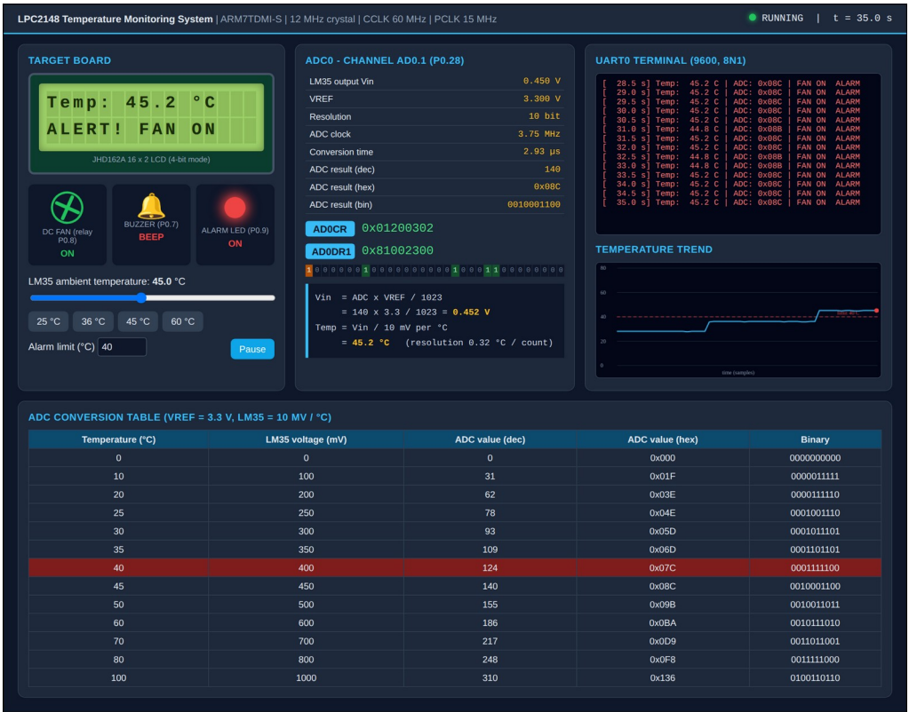
Fig. 3 - ADC = 0x08C (140); LCD shows ALERT! FAN ON; the fan rotates, the buzzer sounds and the alarm LED glows.
