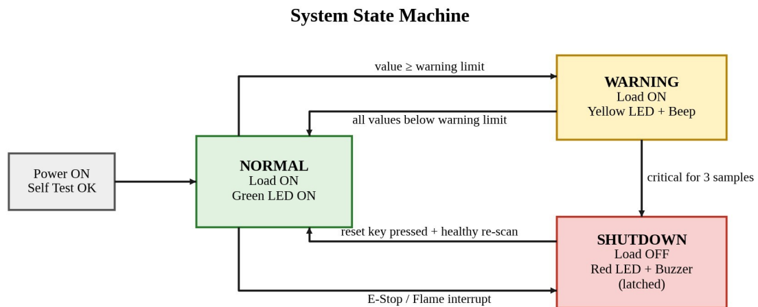
Figure 32: System state machine (NORMAL, WARNING, SHUTDOWN)
