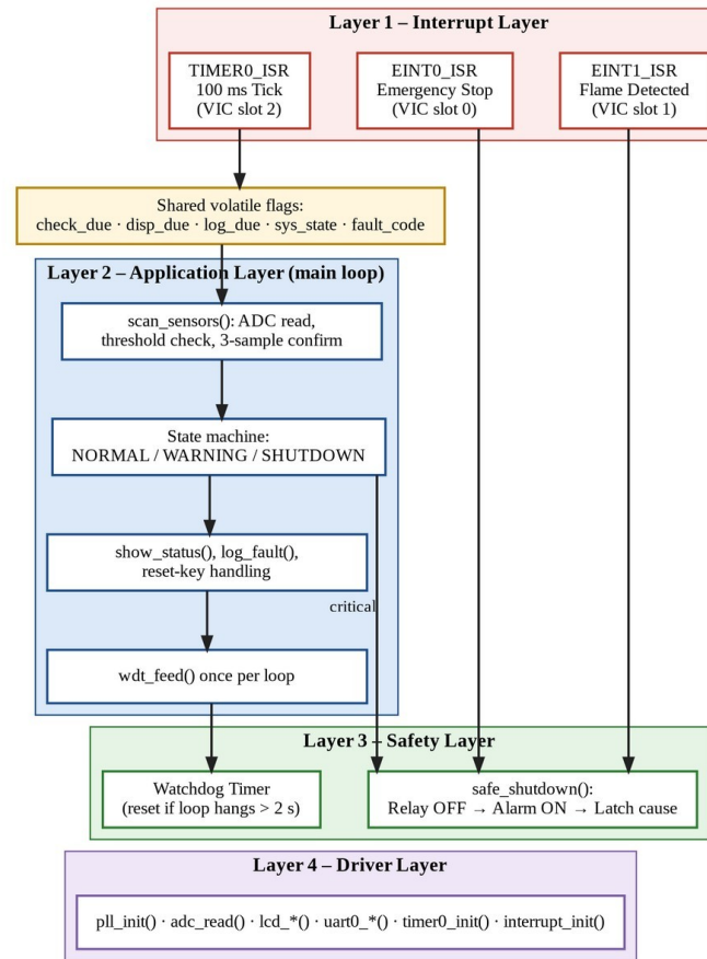
Layered Software Structure of the Fault Detection Firmware
