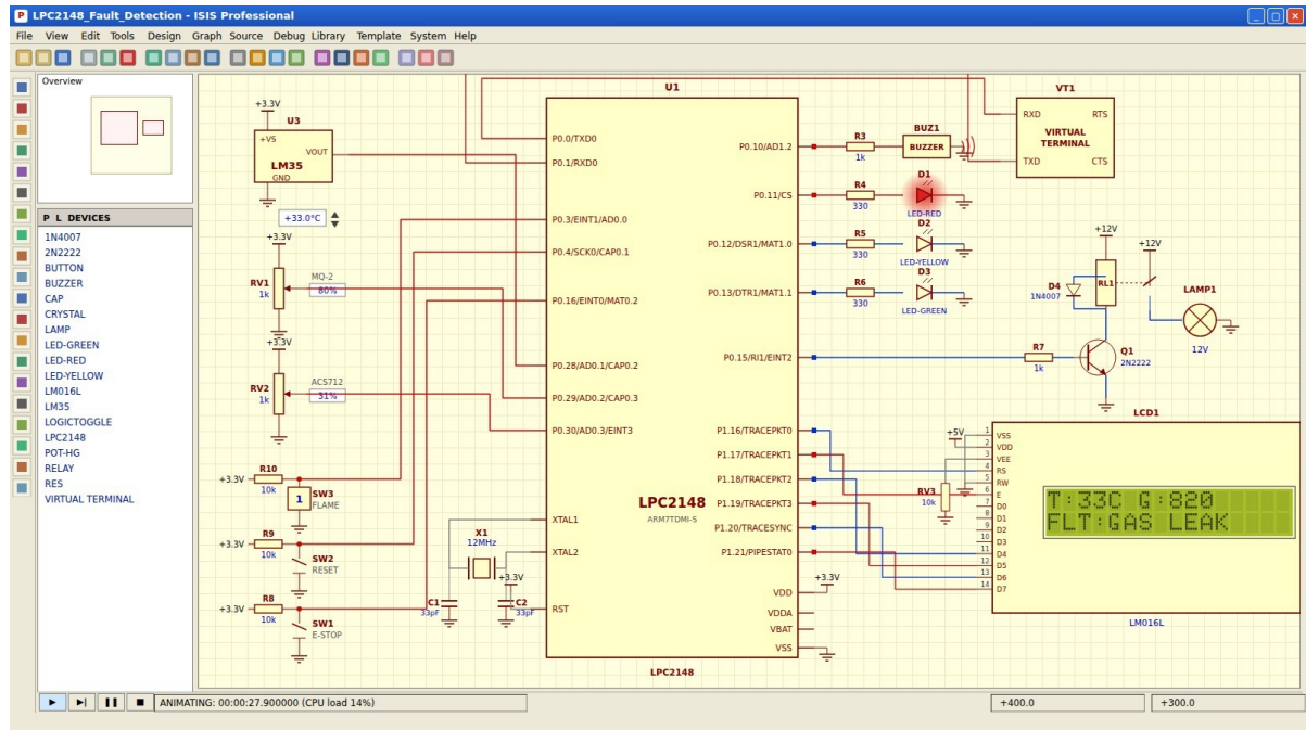
Figure 21: Proteus – load OFF after the gas potentiometer exceeds 800 counts
