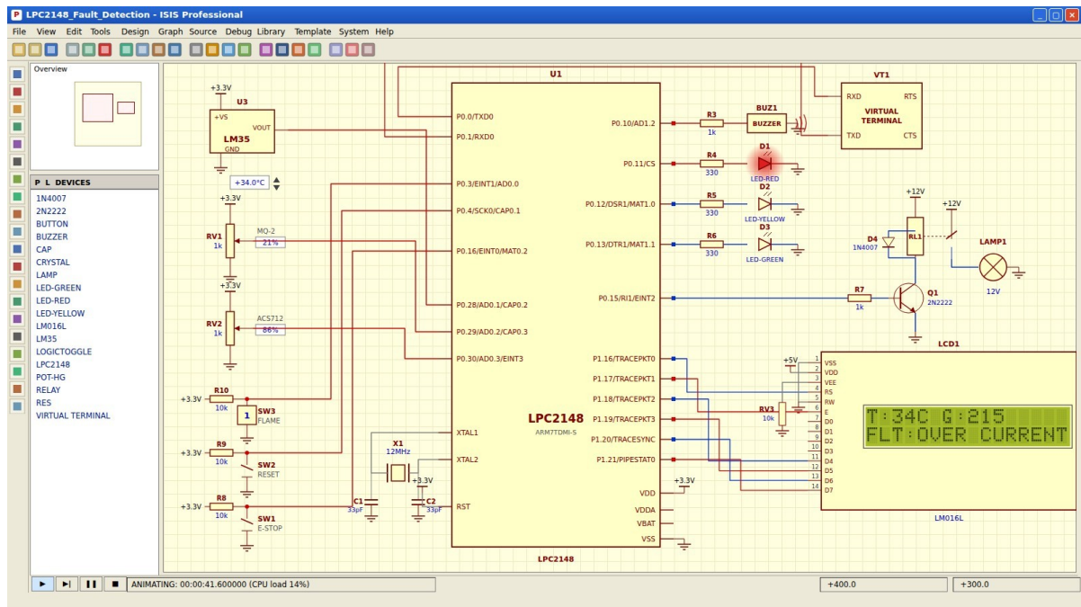
Figure 23: Proteus – load OFF after the current potentiometer exceeds 850 counts
