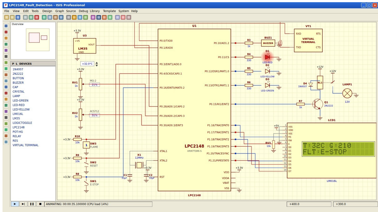
Figure 25: Proteus – E-stop pressed, load OFF immediately, LCD shows FLT:E-STOP
