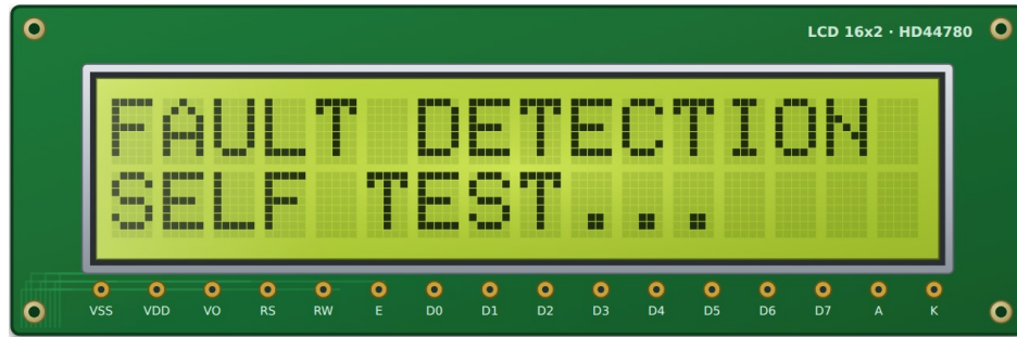
Figure 12: LCD module at start-up
