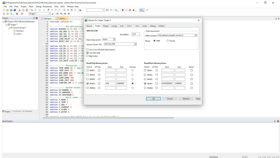
Figure 6: Options for Target – Xtal (MHz) = 12.0
