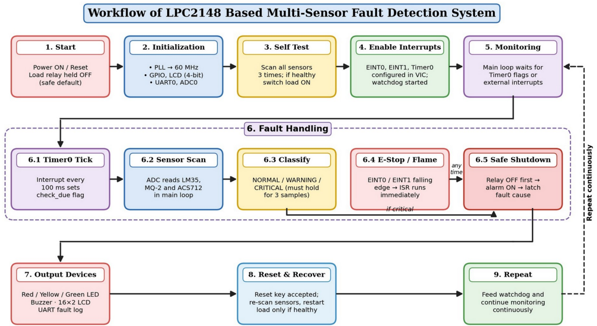
Figure 1: Workflow of the LPC2148 Based Multi-Sensor Fault Detection System
