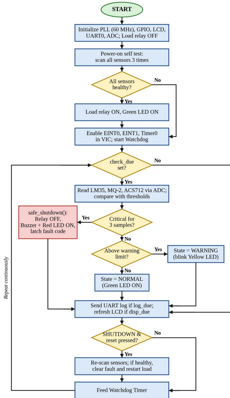
Flowchart of LPC2148 Based Fault Detection System
