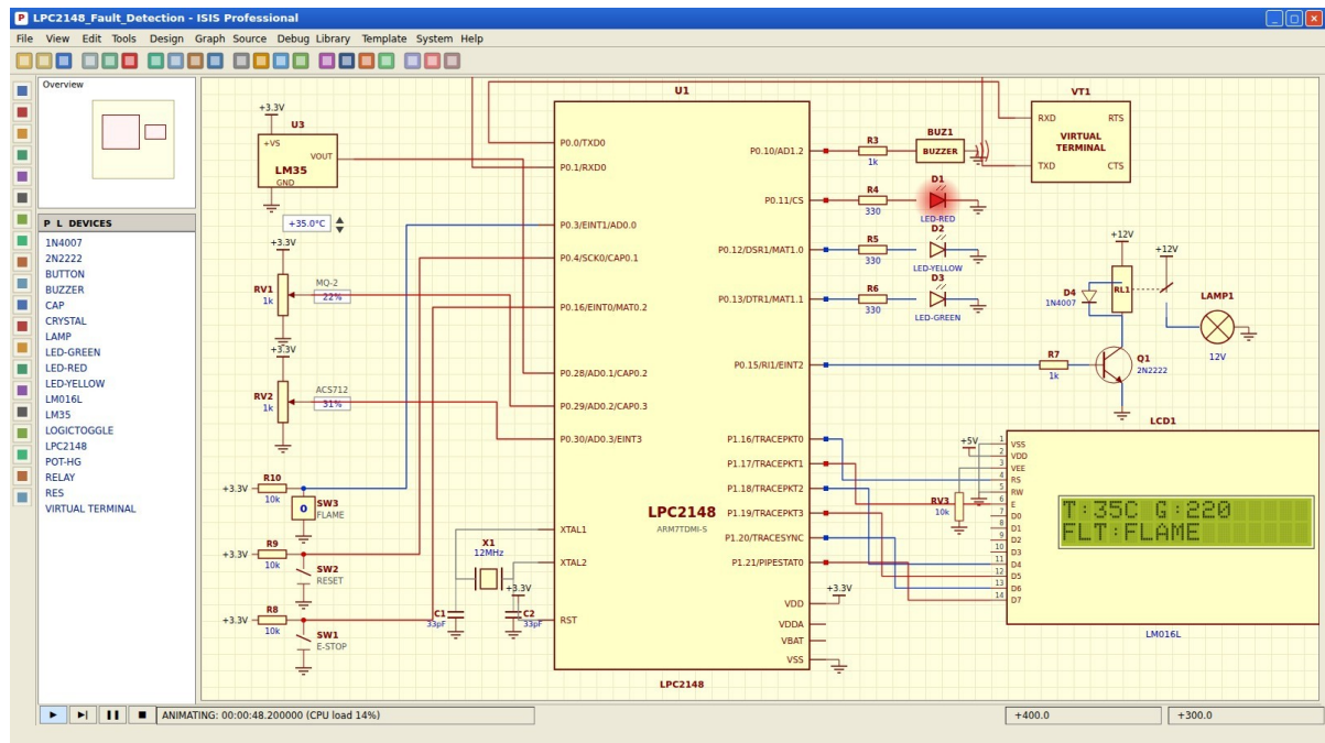
Figure 27: Proteus – flame input pulled low, load OFF immediately
