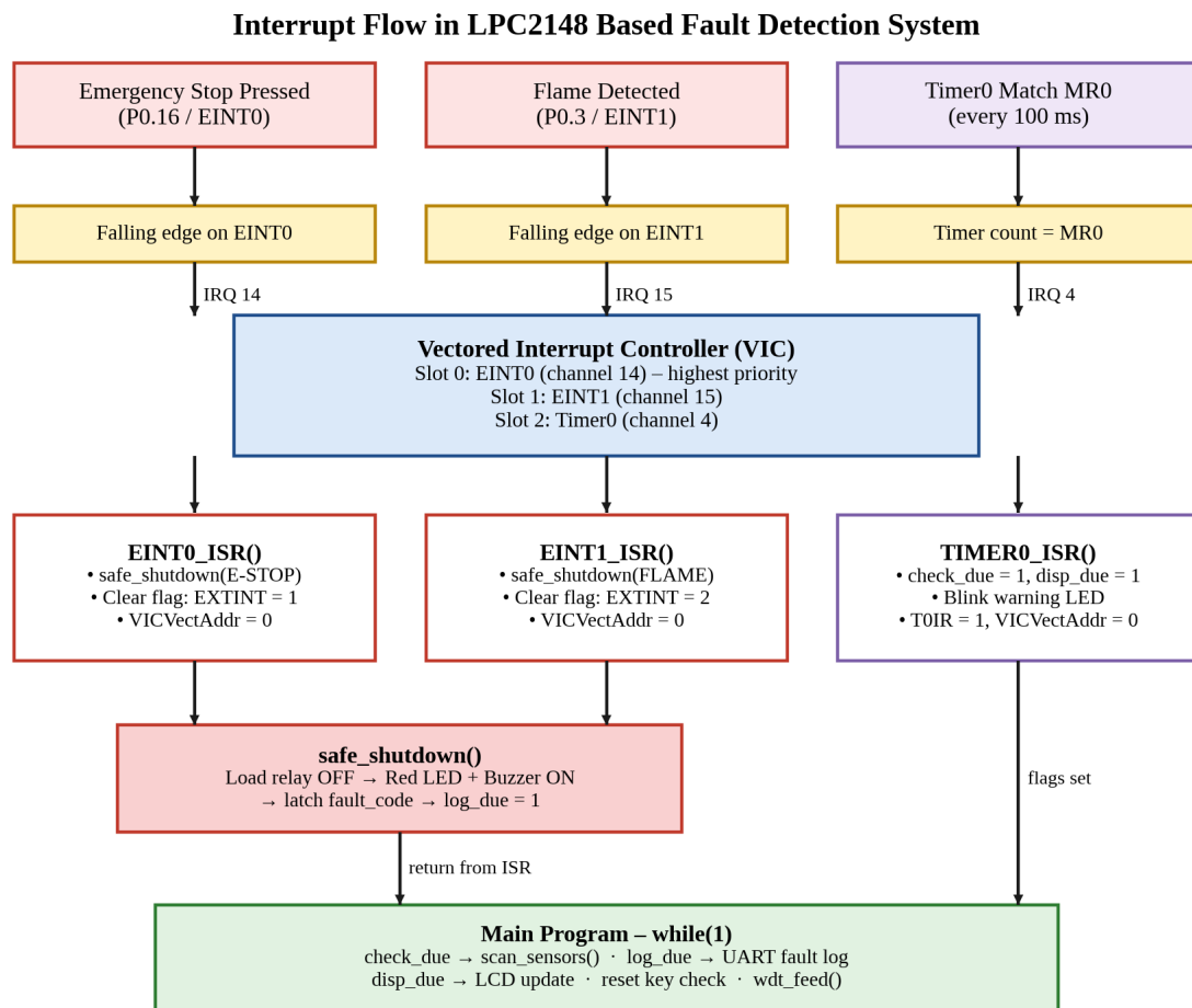
Figure 31: Interrupt flow in the LPC2148 based fault detection system
