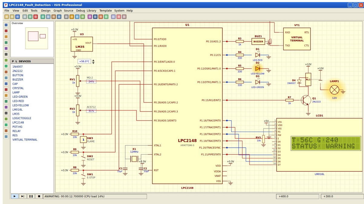
Figure 17: Proteus – load ON, yellow LED blinking, buzzer beeping
