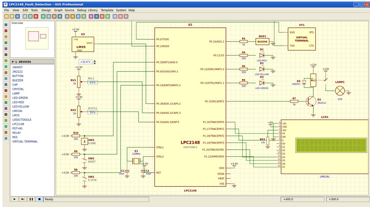
Figure 10: ISIS schematic of the LPC2148 based fault detection system (simulation not started)
