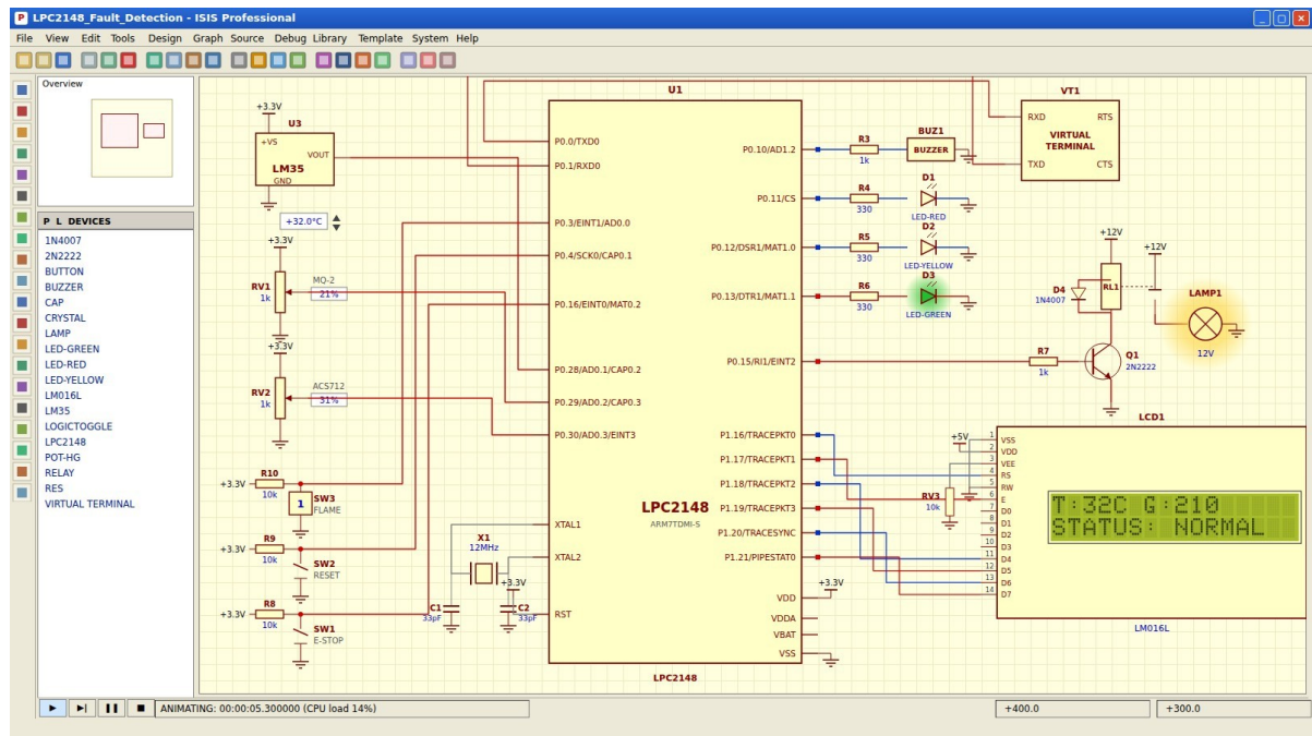
Figure 15: Proteus – load lamp ON, green LED ON
