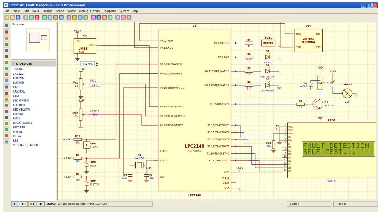
Figure 13: Proteus – self test running, load still OFF
