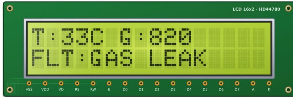
Figure 20: LCD module – T:33C G:820 / FLT:GAS LEAK
