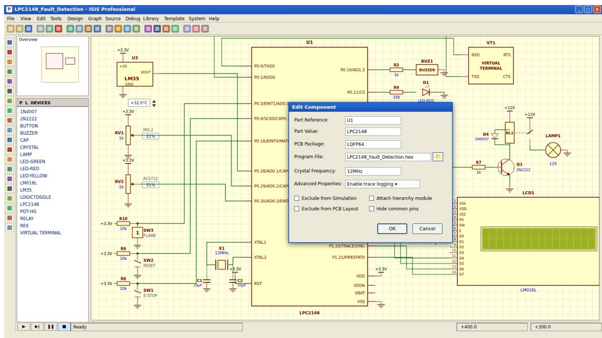
Figure 11: Edit Component dialog of U1 – Program File = LPC2148_Fault_Detection.hex, clock 12 MHz
