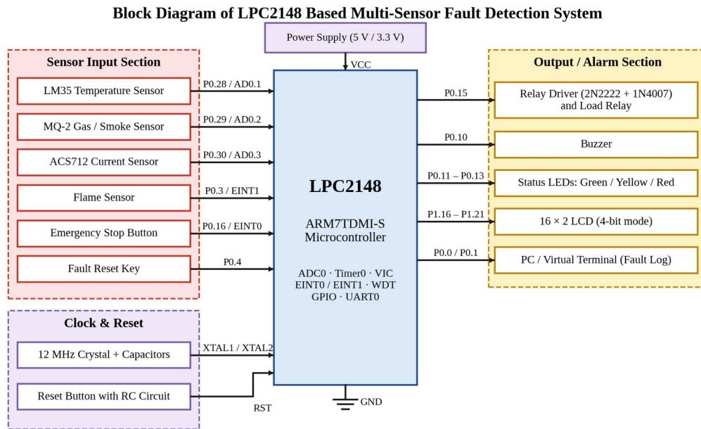
Figure 29: Block diagram of the LPC2148 based multi-sensor fault detection system
