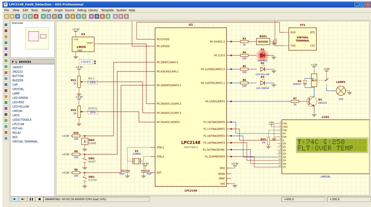
Figure 19: Proteus – load lamp OFF, red LED and buzzer ON
