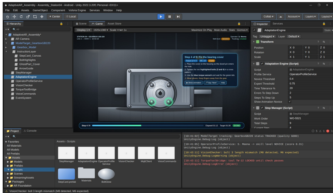
Fig. 11 - Play mode: the Game view shows the AR overlay for the novice operator while the Console logs the checks.
