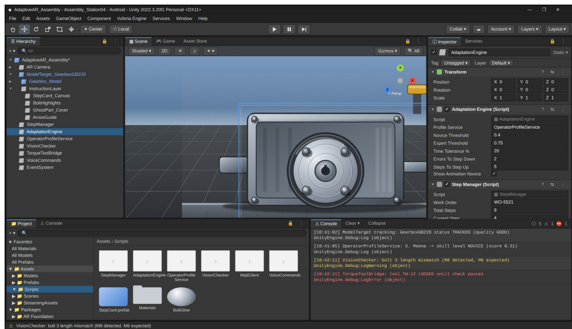
Fig. 10 - Unity editor (Scene view) with the Model Target, the instruction layer, the Adaptation Engine settings and the console log of one step.
