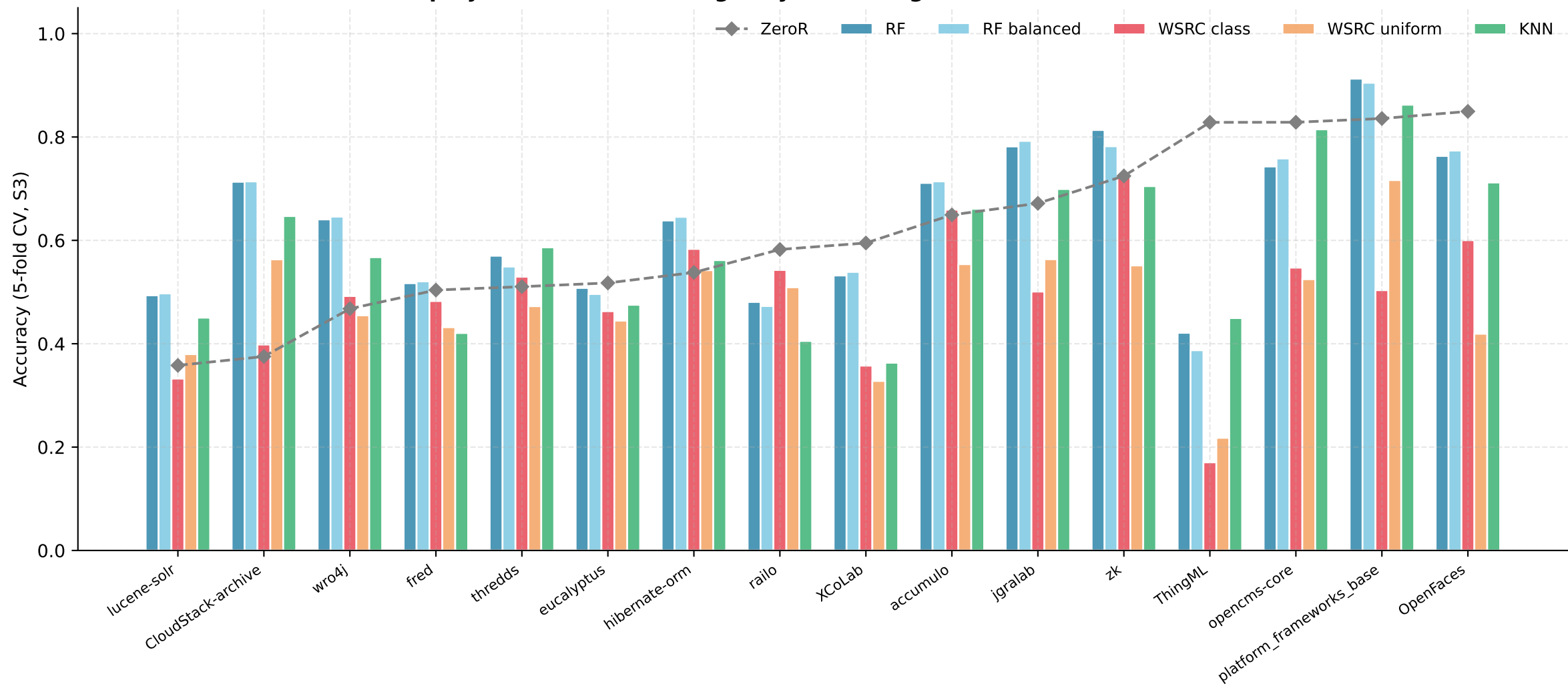
Per-Project Accuracy — Standard Training (projects ordered left→right by increasing class imbalance / ZeroR)
