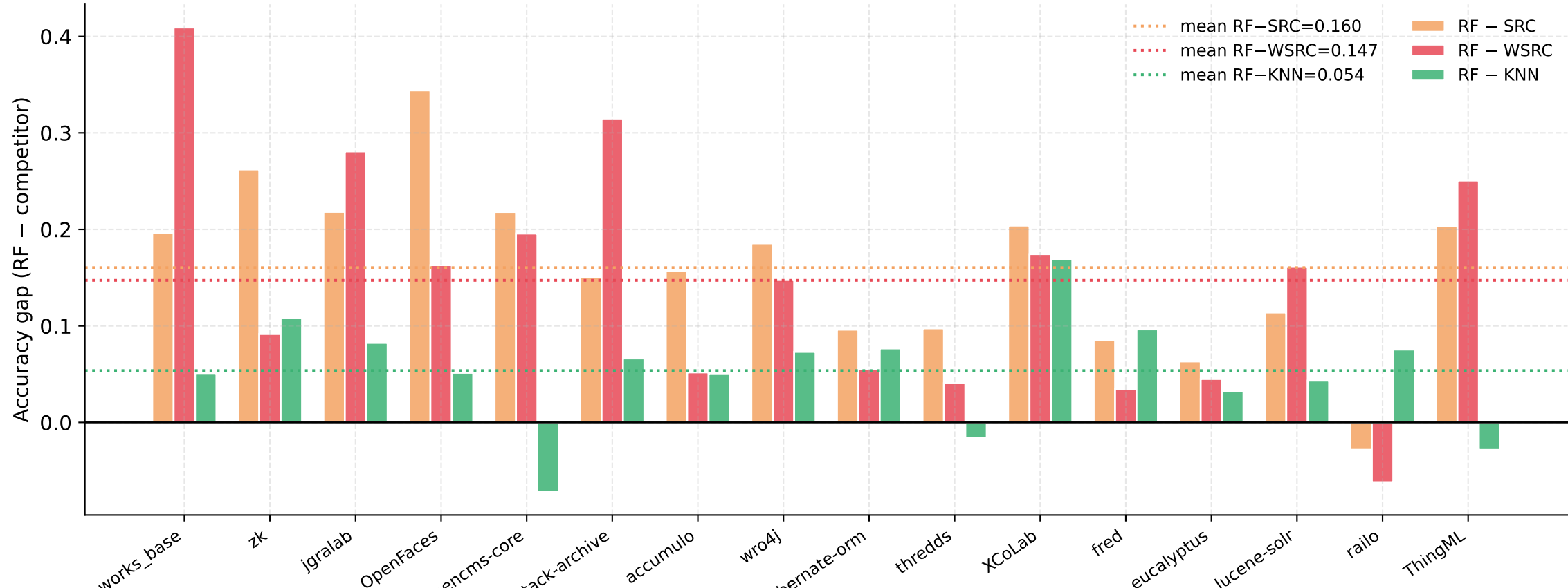
RF Accuracy Advantage over SRC, WSRC, and KNN per Project
