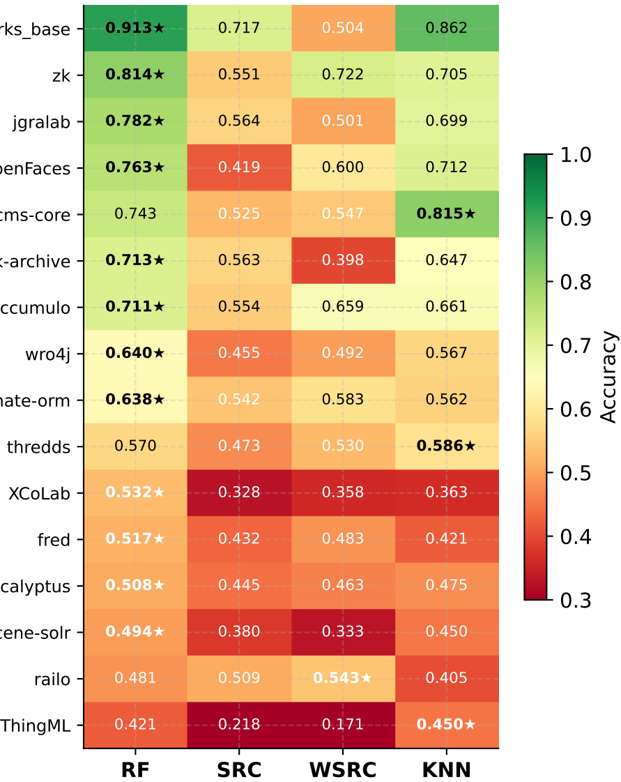
Accuracy Heatmap: RF vs. SRC vs. WSRC per Project
