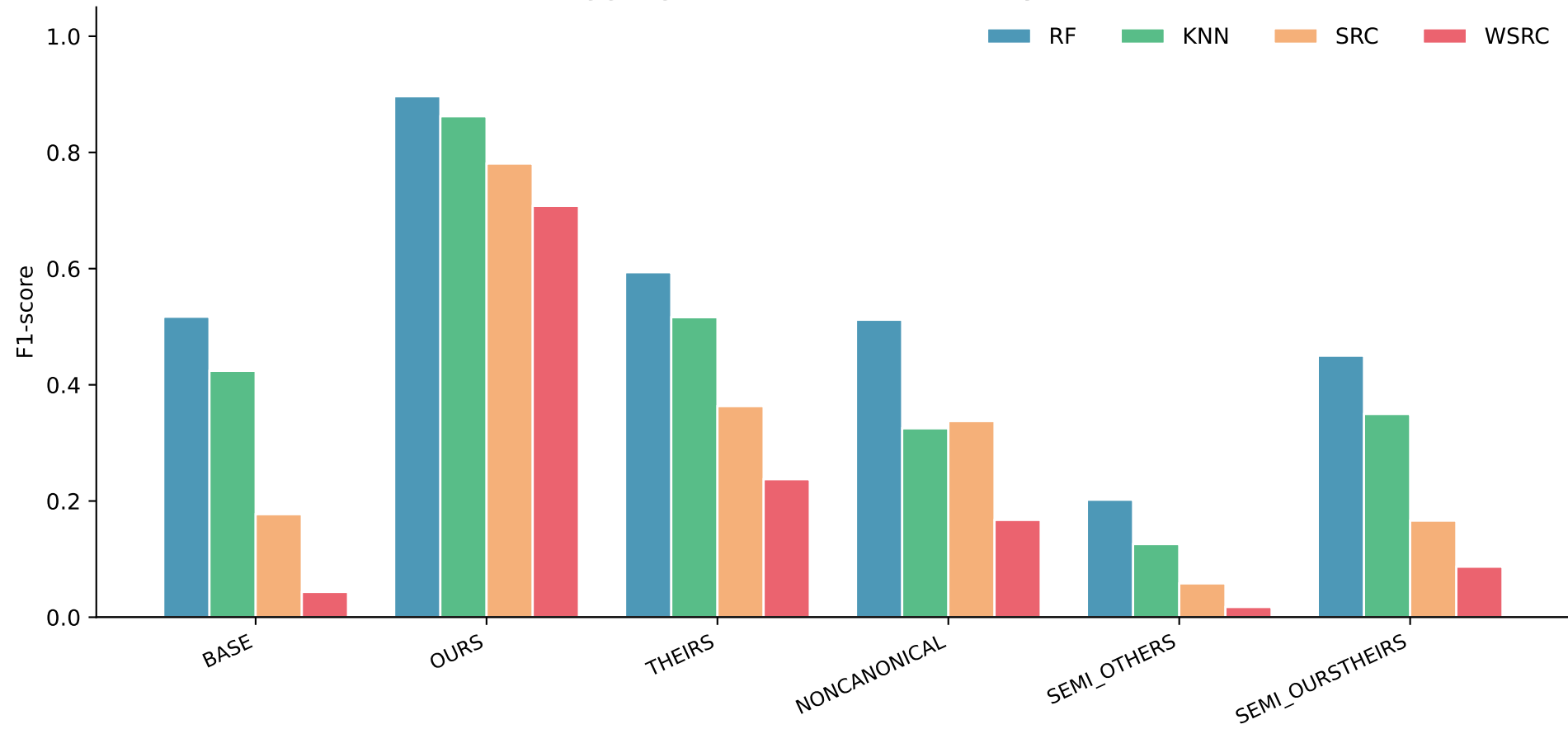
Per-Class F1-Score by Model (aggregated across all 16 projects)
