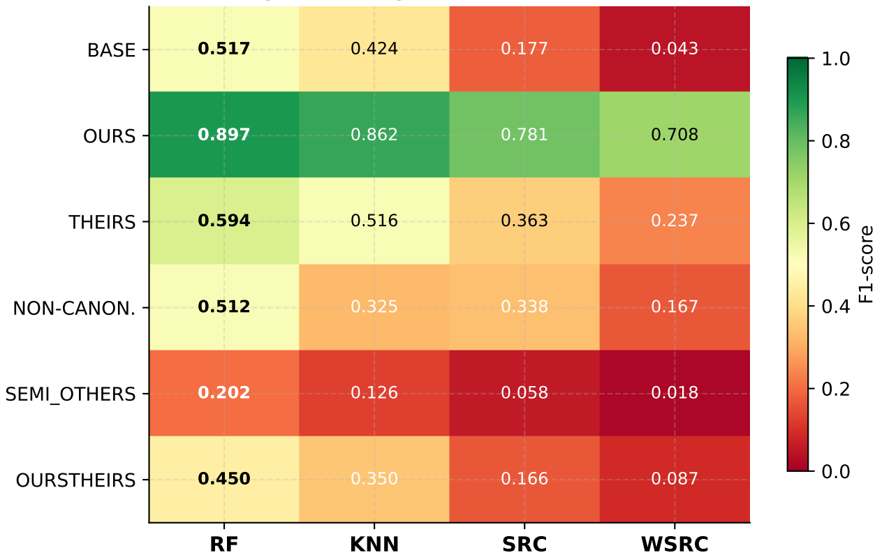
F1-Score Heatmap: Class × Model (green = high F1, red = low F1)
