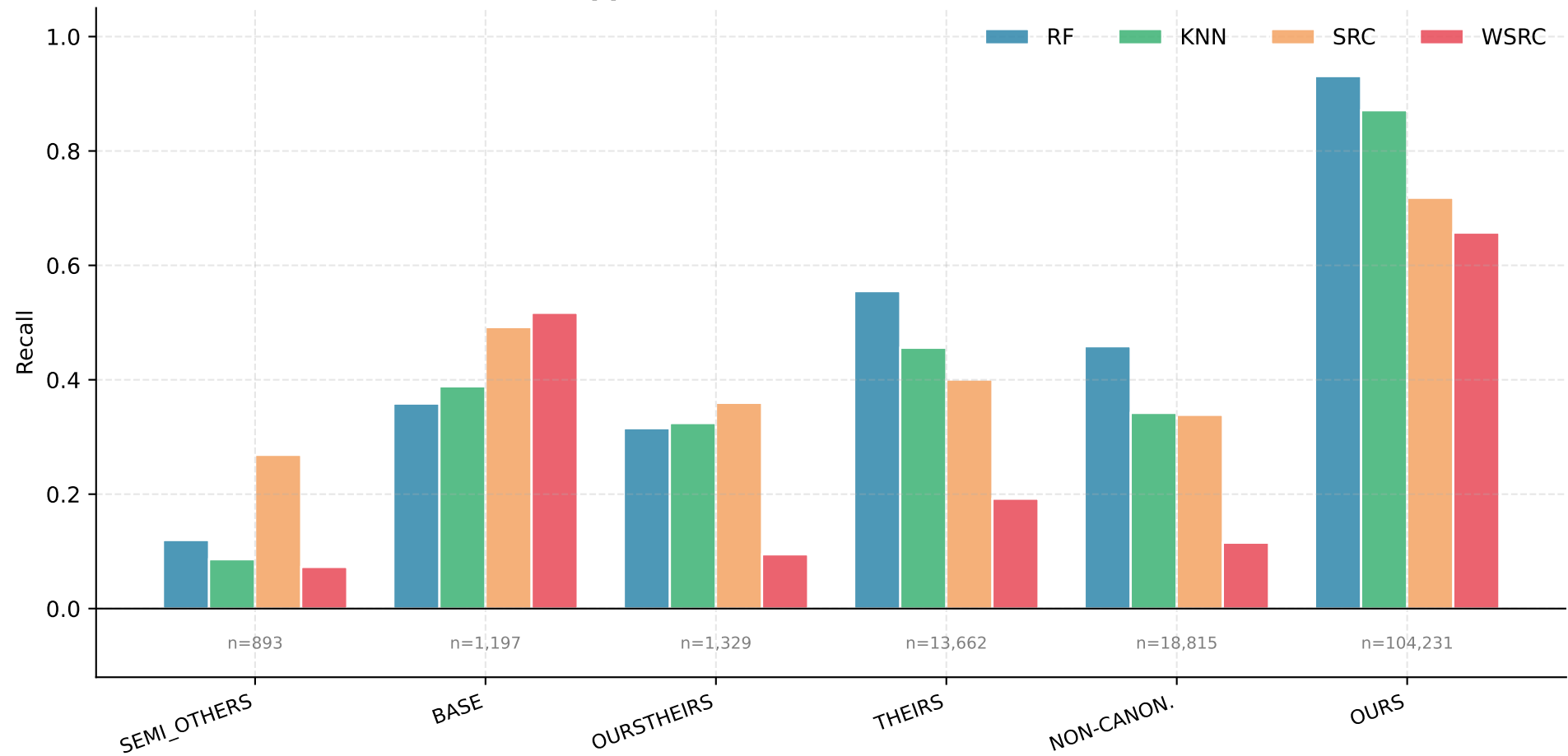
Per-Class Recall by Model (classes ordered by frequency, rarest left) Support (n=) shown below each class
