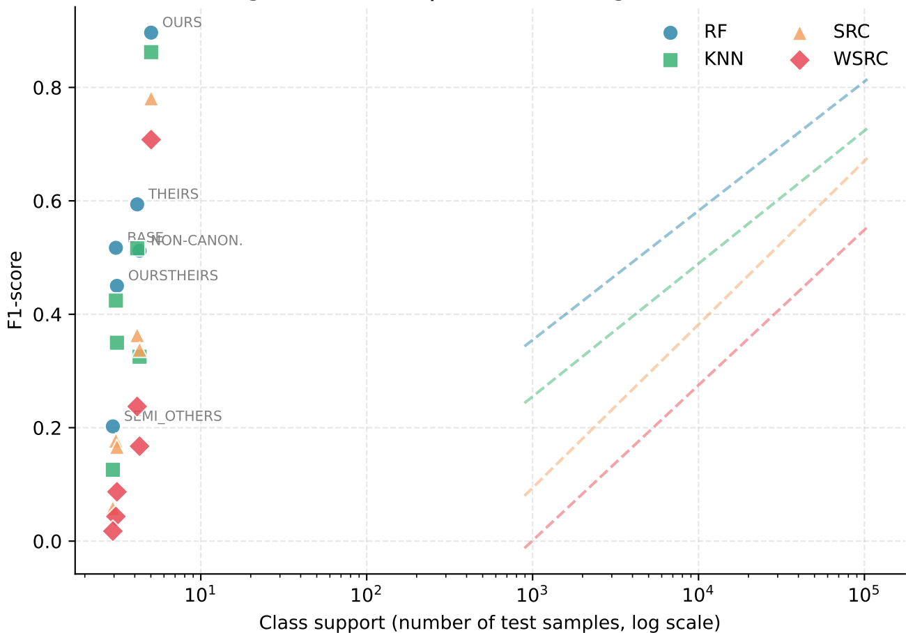
F1-score vs. Class Frequency (dashed = log-linear trend | all models degrade on rare classes)
