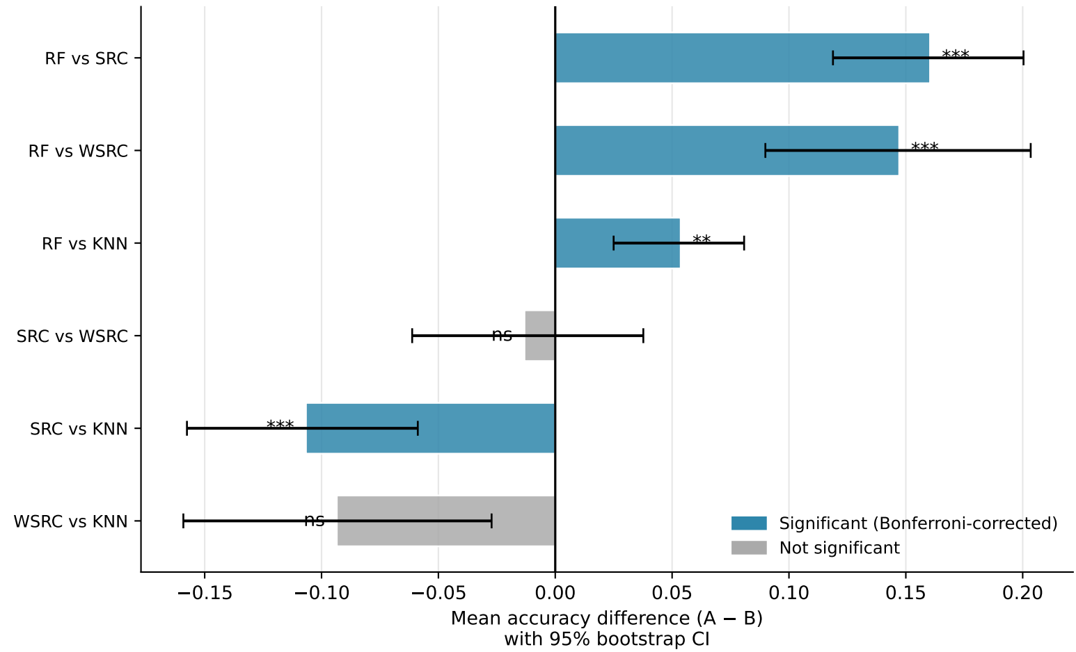
Effect Sizes: Pairwise Accuracy Differences (blue = significant after Bonferroni; gray = not significant)
