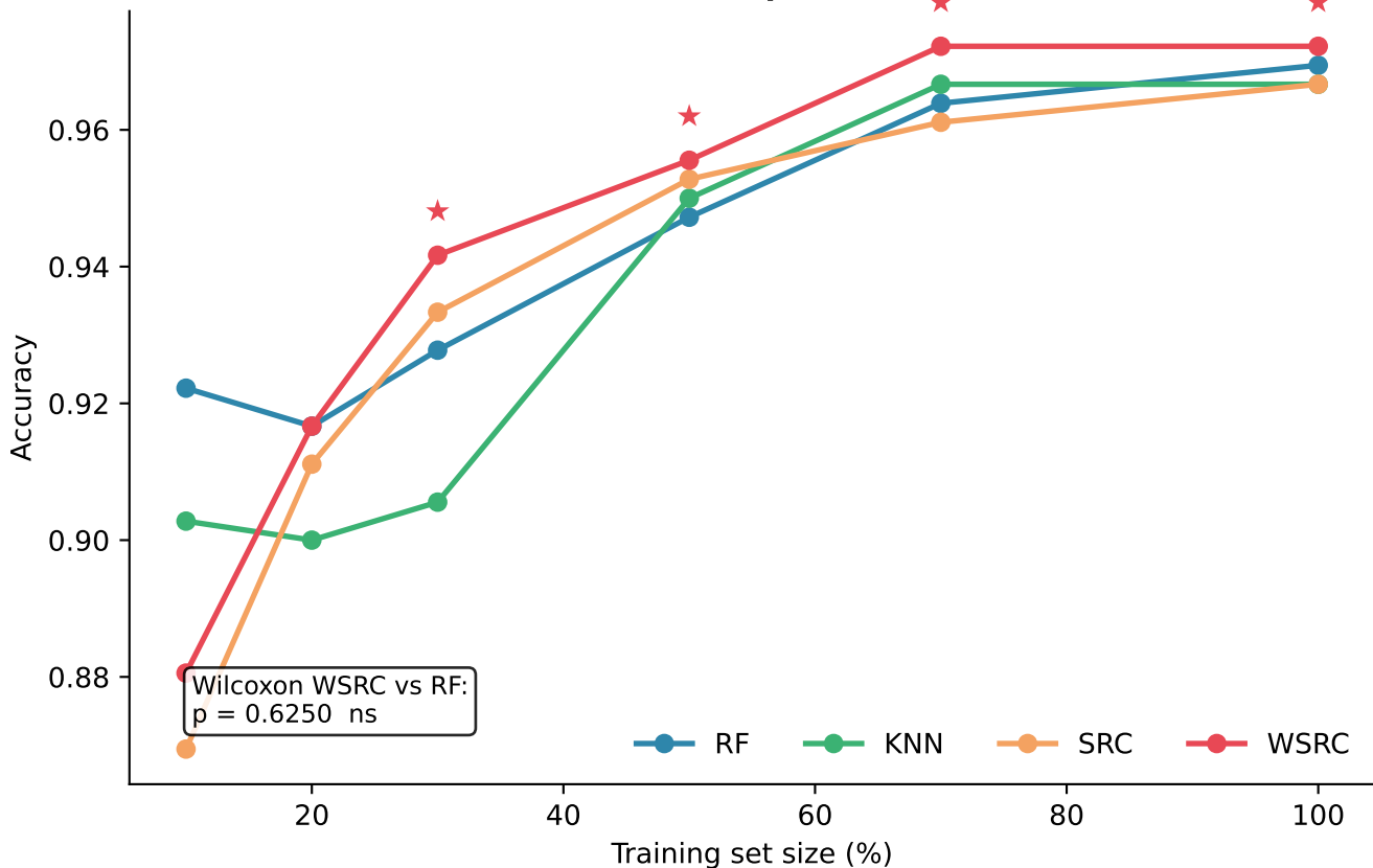
Digits Dataset — Learning Curve (★ = WSRC > RF at this training size; Wilcoxon test over all points shown in box)
