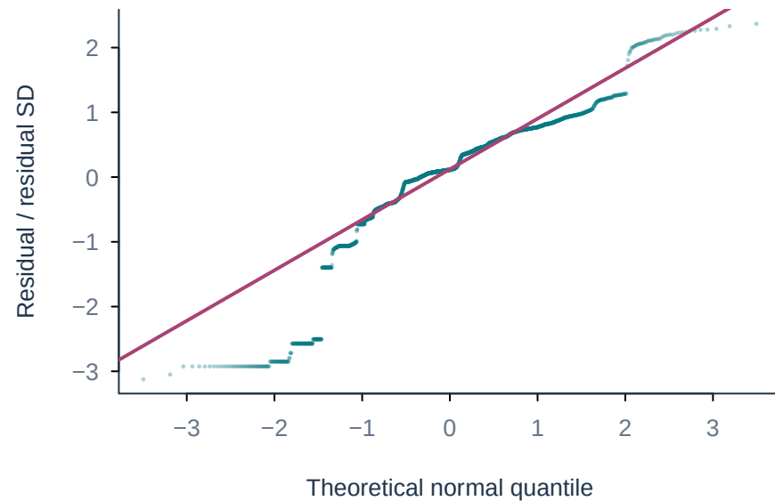
LogSKR : normal Q-Q
