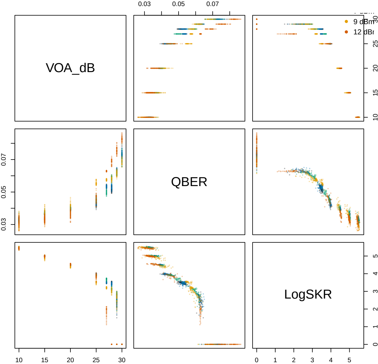
Scatterplot Matrix of QKD Performance Variables
