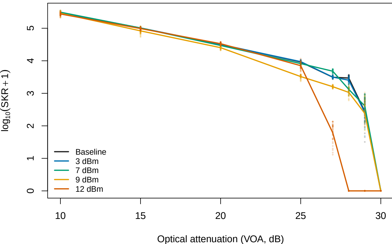
Secure Key Rate Across Attenuation and Noise Conditions
