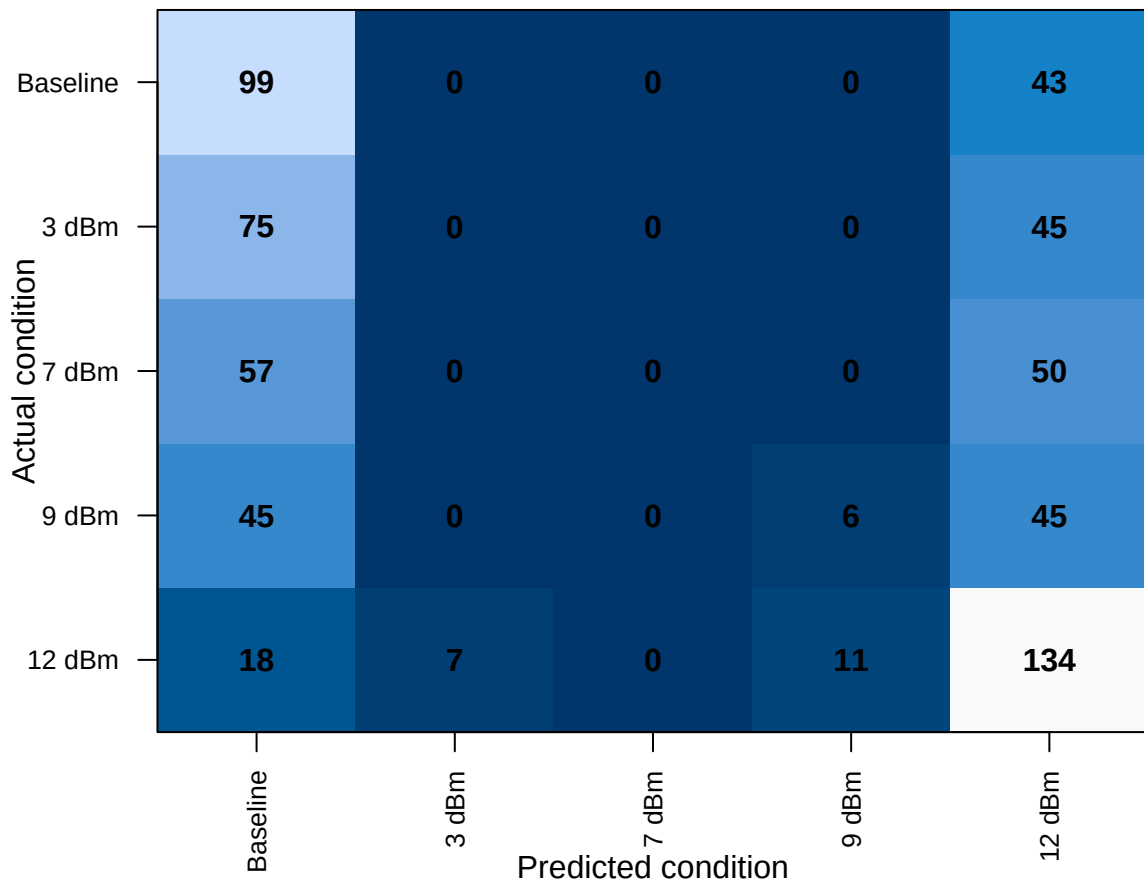
LDA Confusion Matrix (Held-out Test Set)
