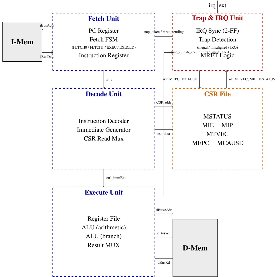
Figure 3.3: CPU Core – Top-Level Functional Block Diagram
