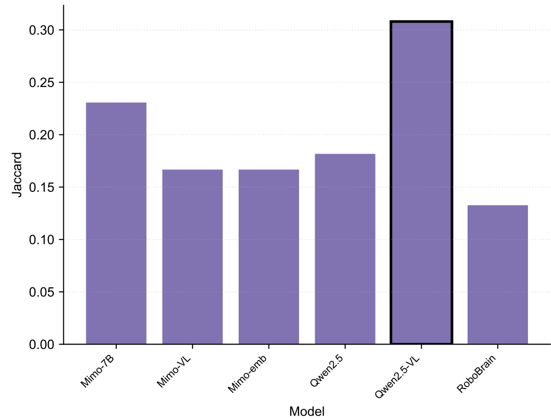
Jaccard
