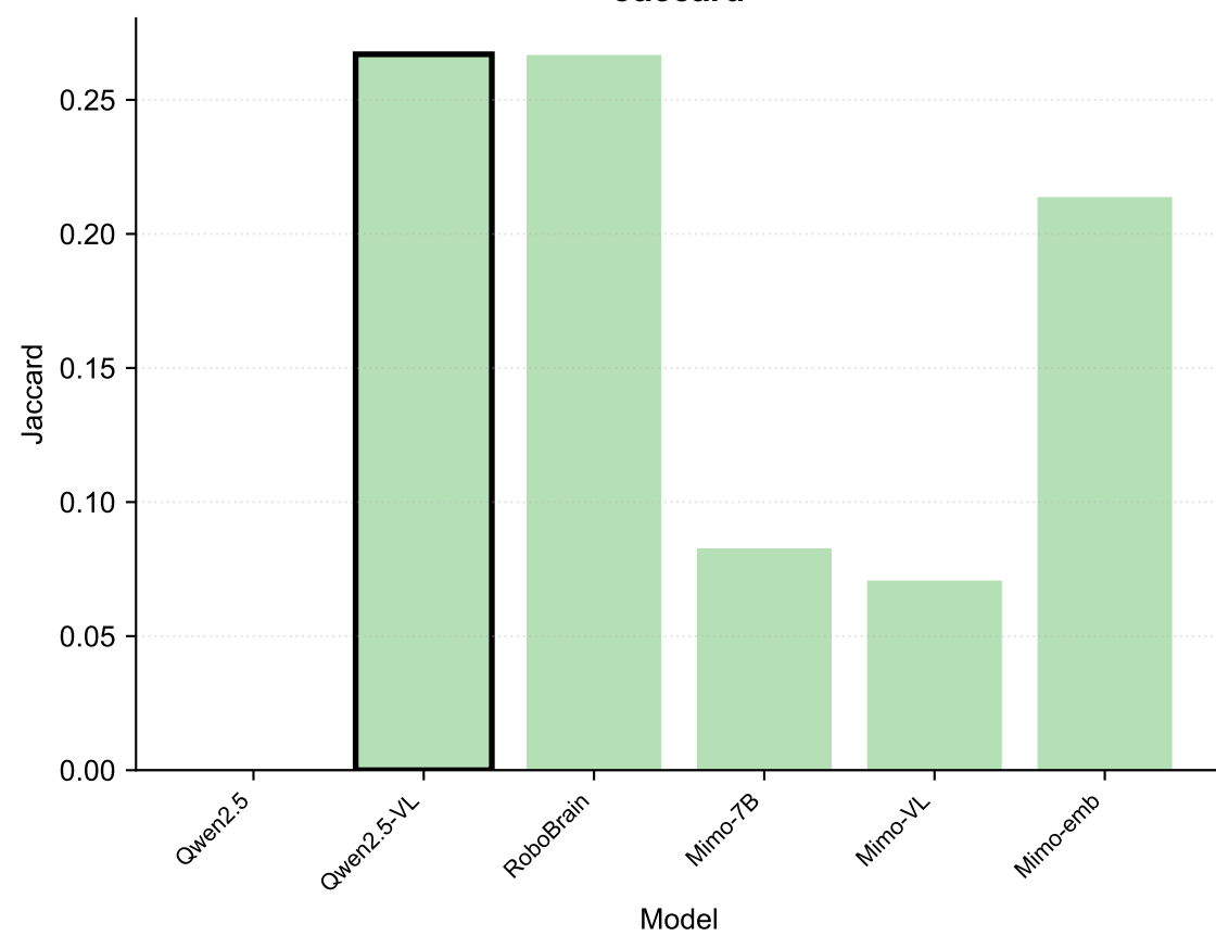
Jaccard
