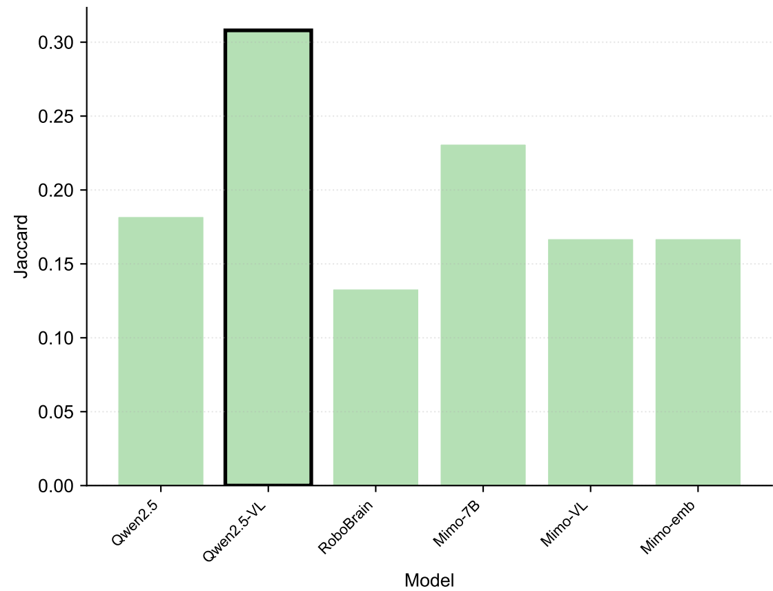
Jaccard
