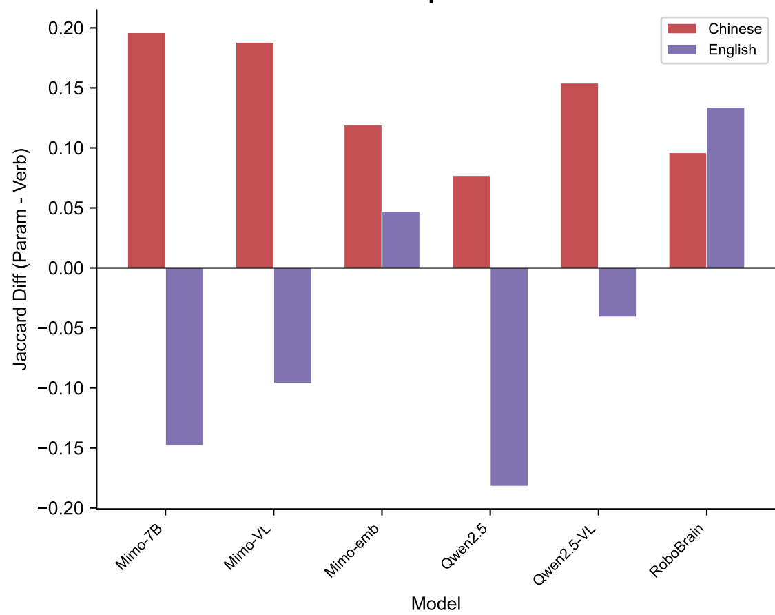
Jaccard: Prompt Format Effect
