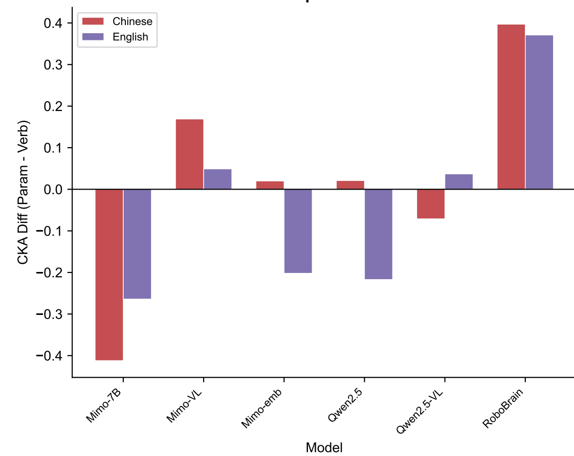
CKA: Prompt Format Effect
