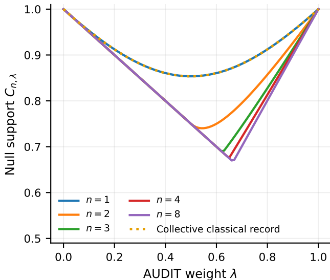
Exact classical-memory supports
