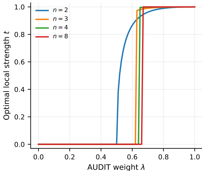
Weak-to-projective strategy transition
